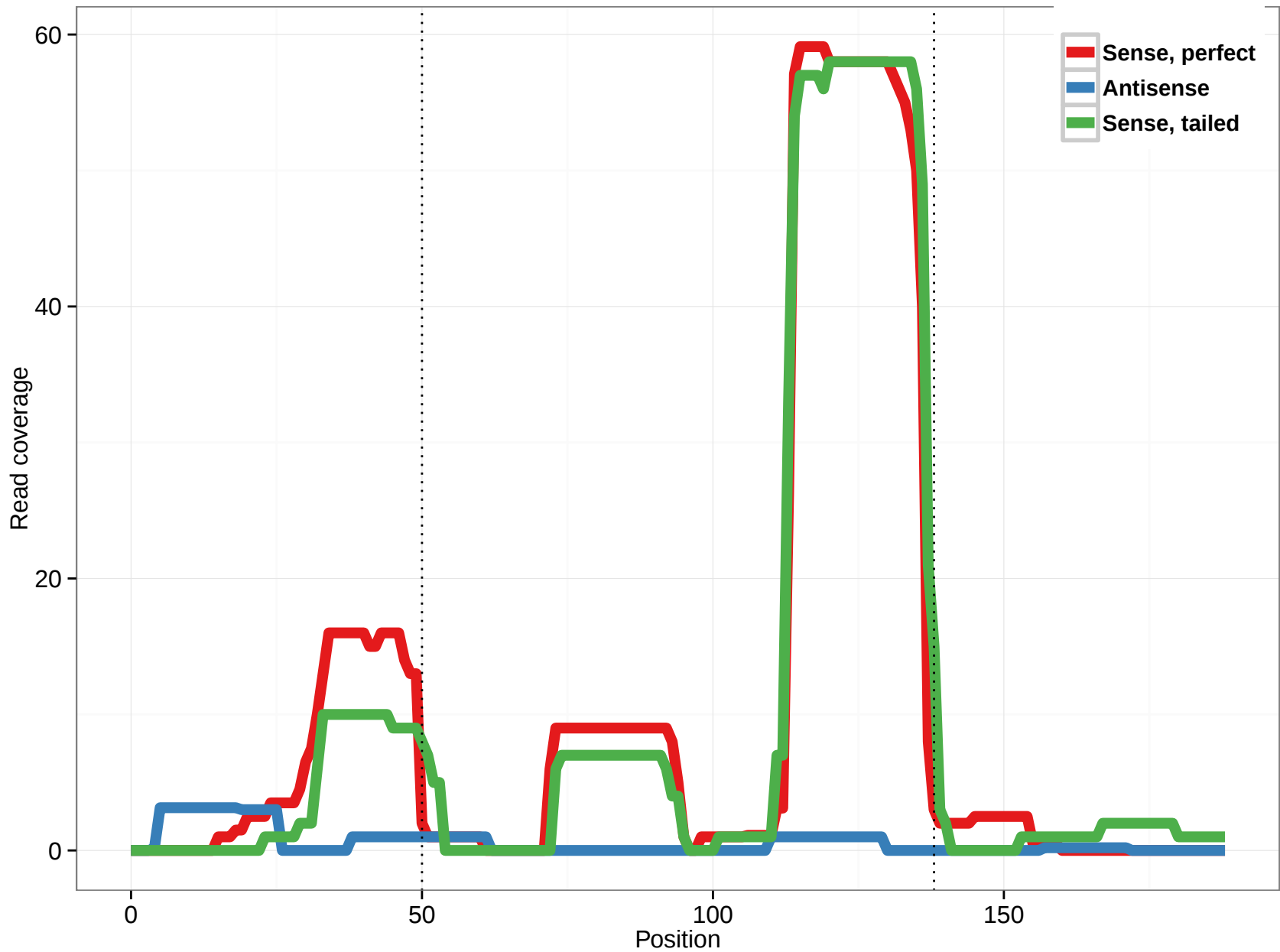
hsa-mir-6743
