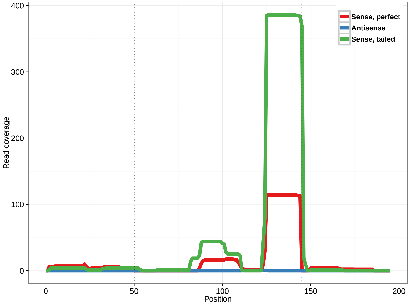
hsa-mir-6742
