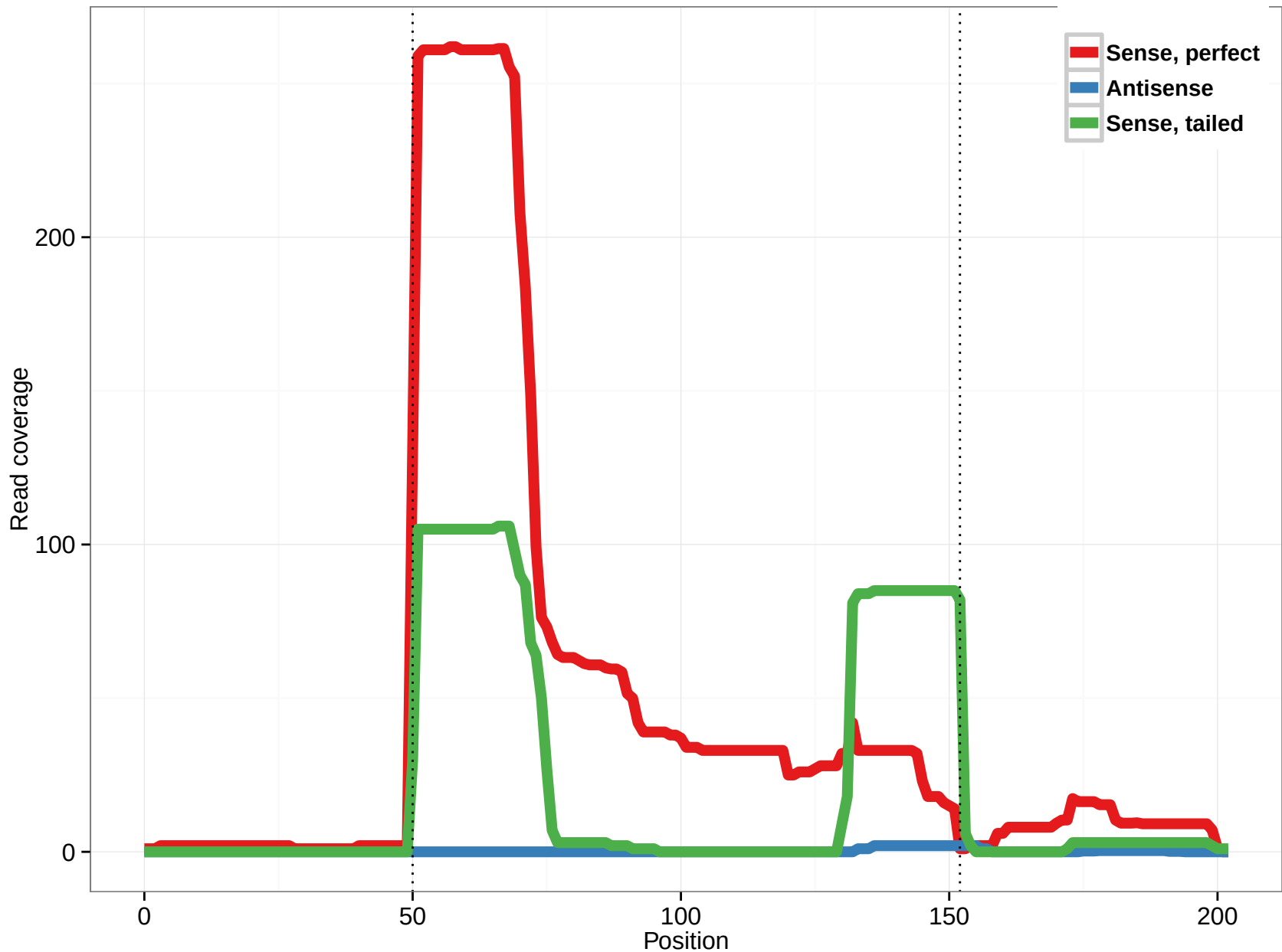
hsa-mir-1236
