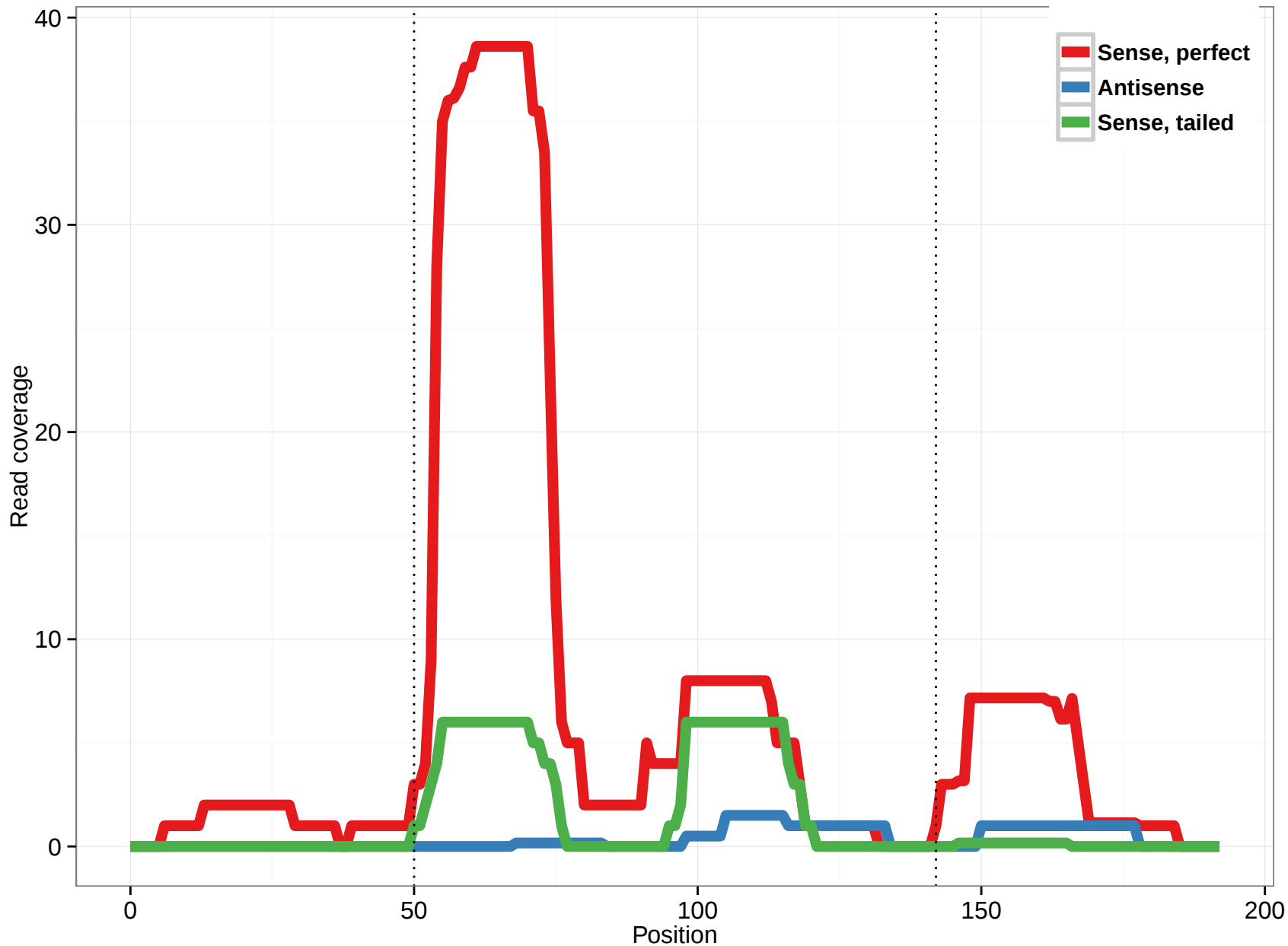
hsa-mir-1231
