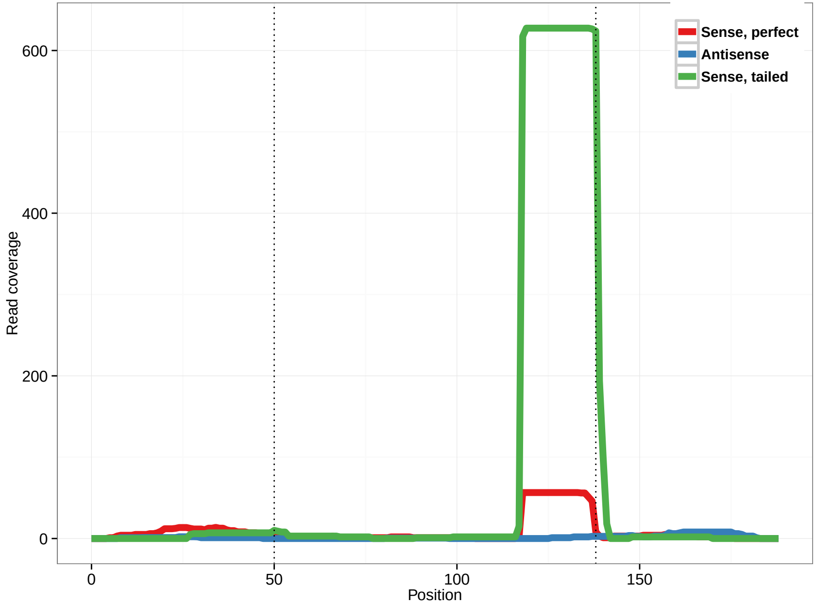
hsa-mir-1227
