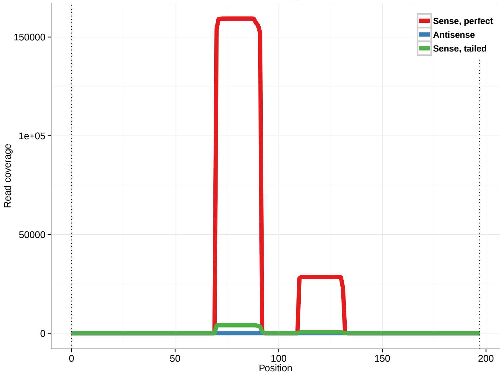
mir-276b
