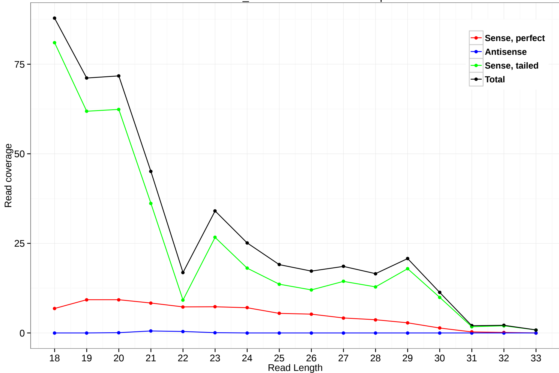
scaffold_4929:9274713-9275485.5p
