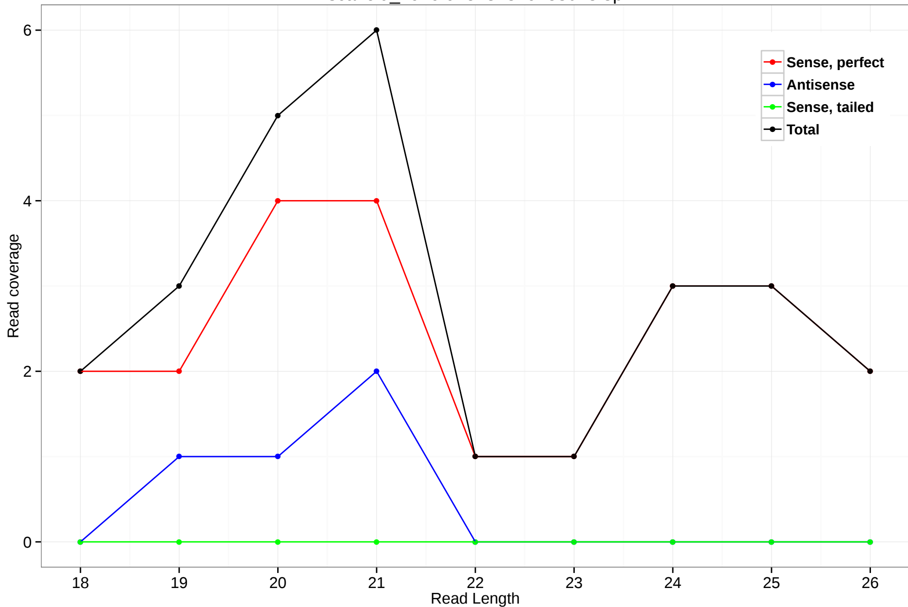
scaffold_4929:9252328-9253043.3p
