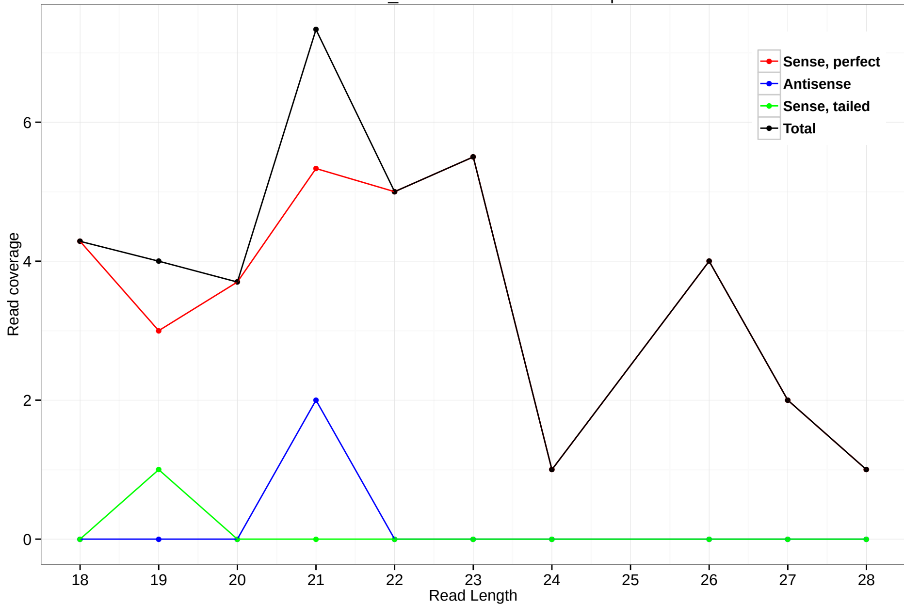
scaffold_4929:9022098-9026179.5p
