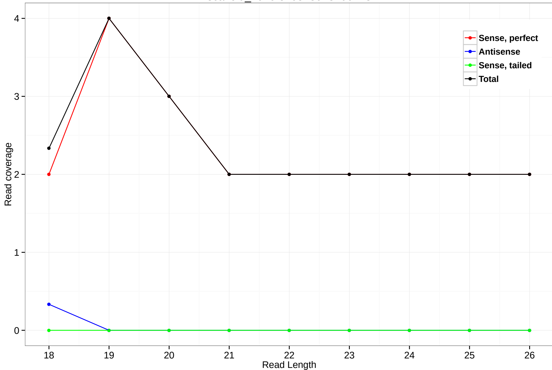
scaffold_4929:8205730-8206148
