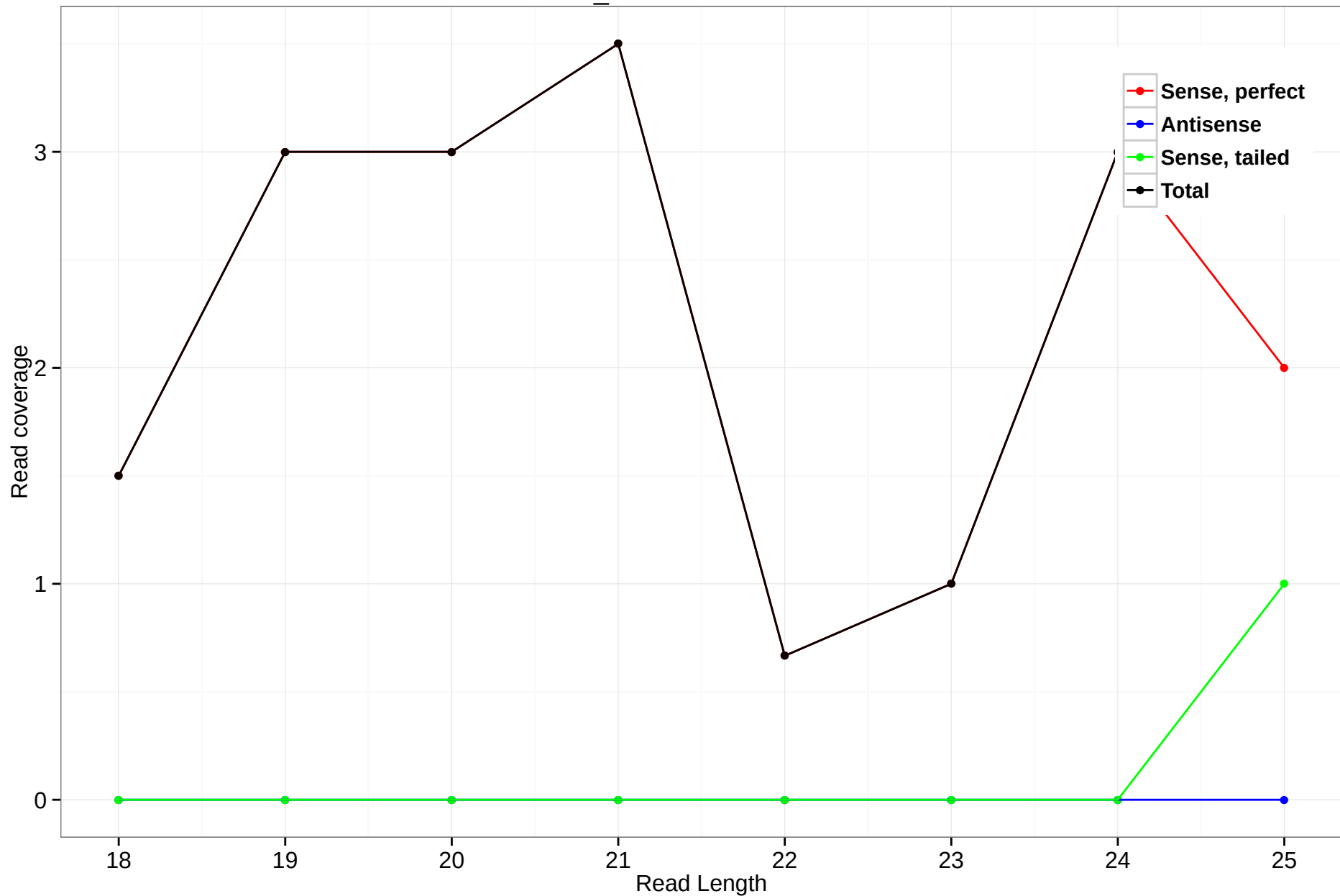
scaffold_4929:6492080-6492288
