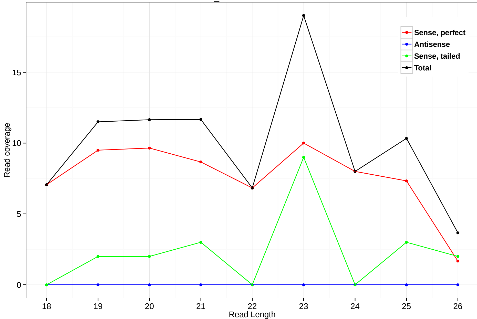
scaffold_4929:6490236-6490396
