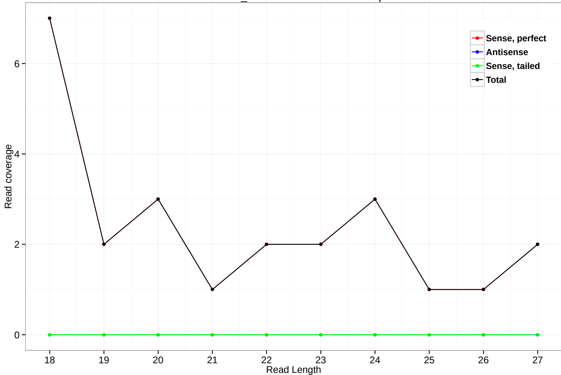
scaffold_4929:6070190-6071492.5p
