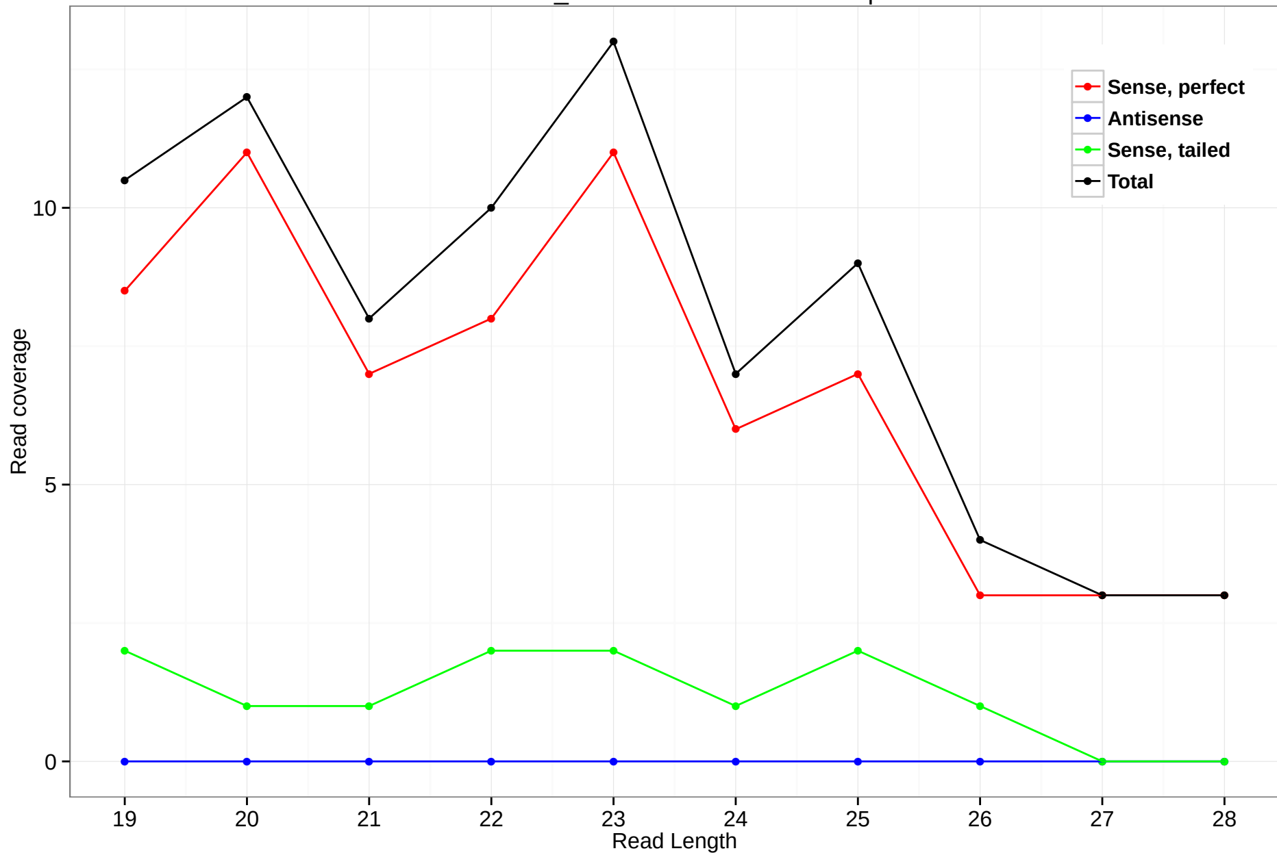
scaffold_4929:6032682-6033315.5p
