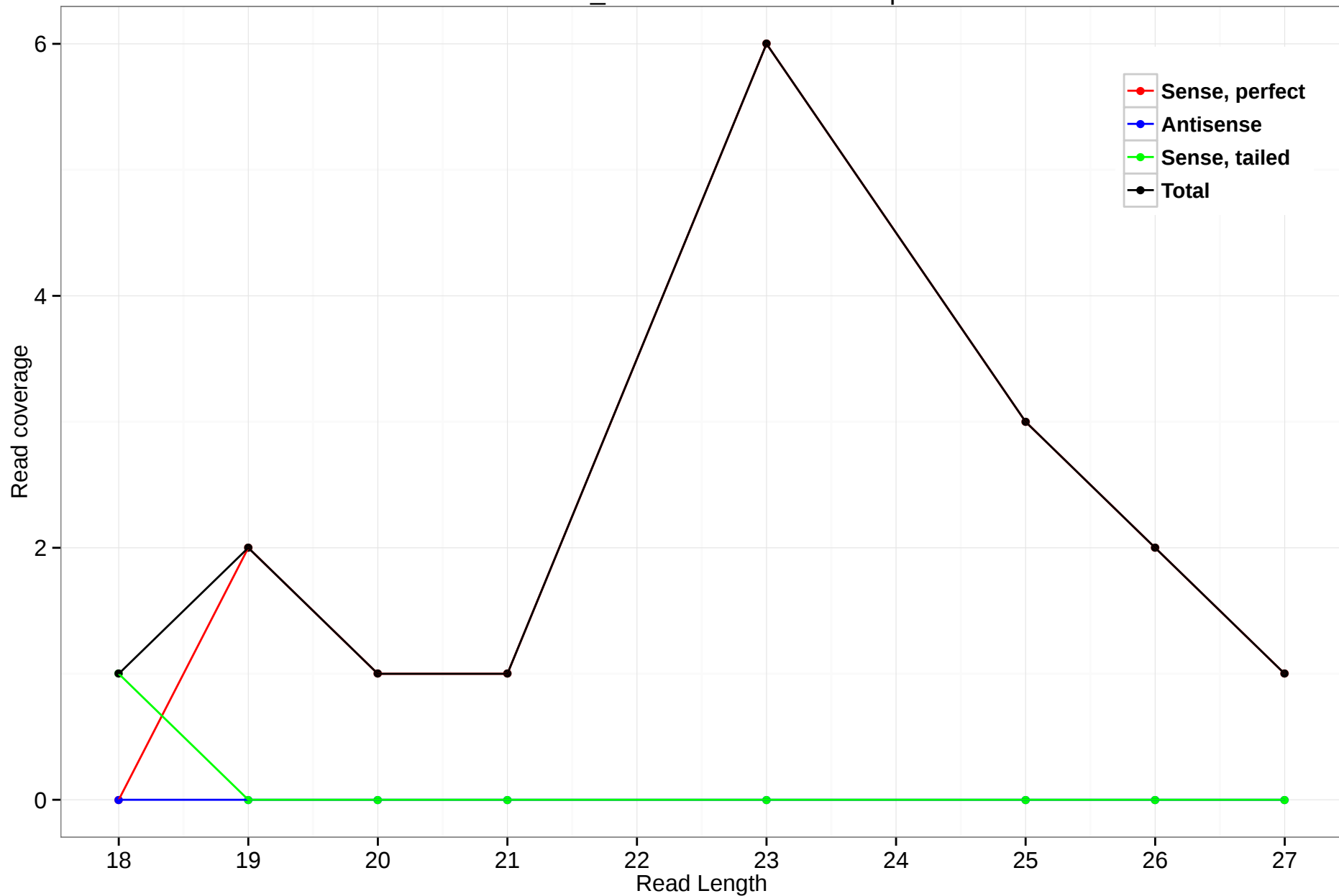
scaffold_4929:596163-596811.5p
