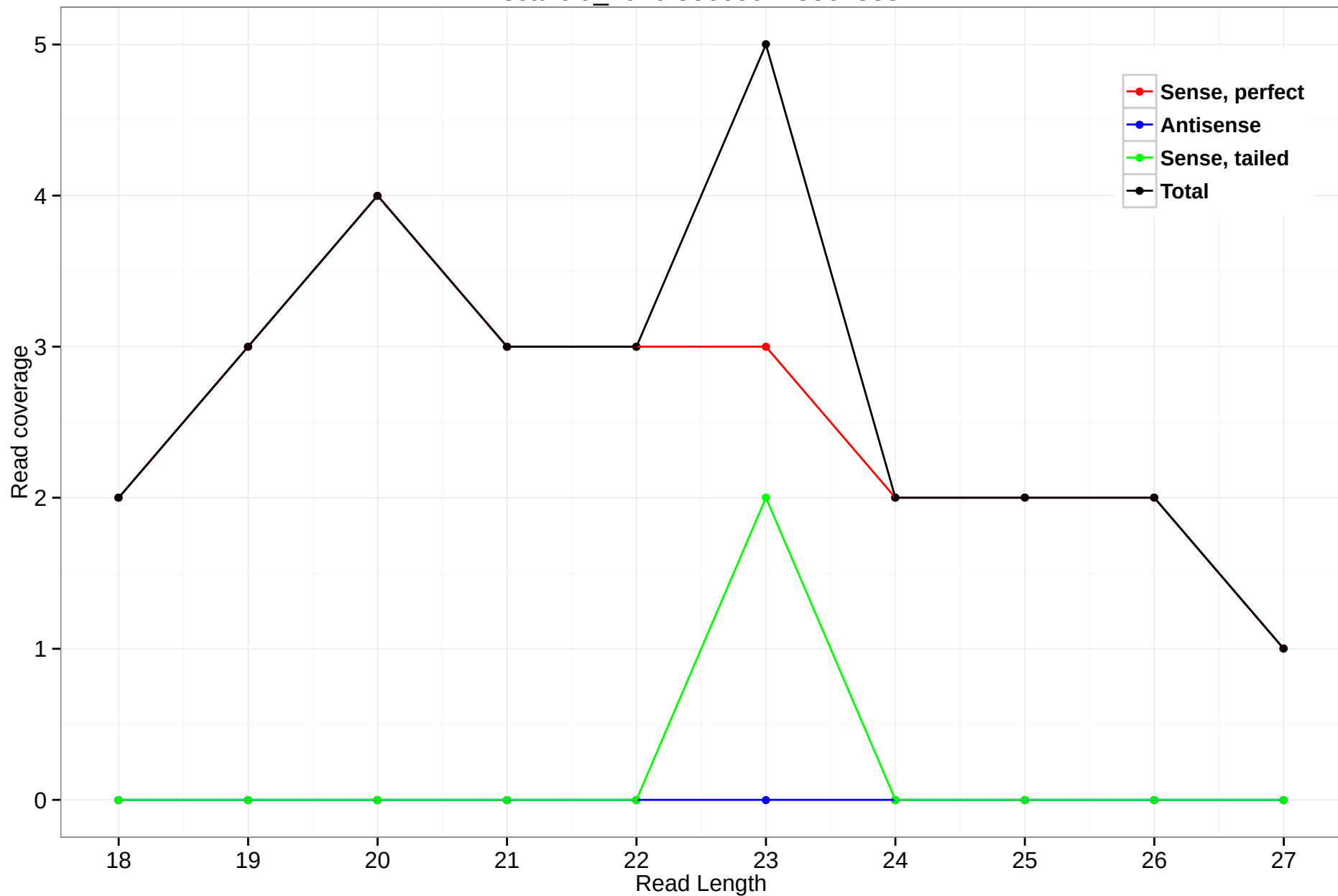
scaffold_4929:5860991-5861333
