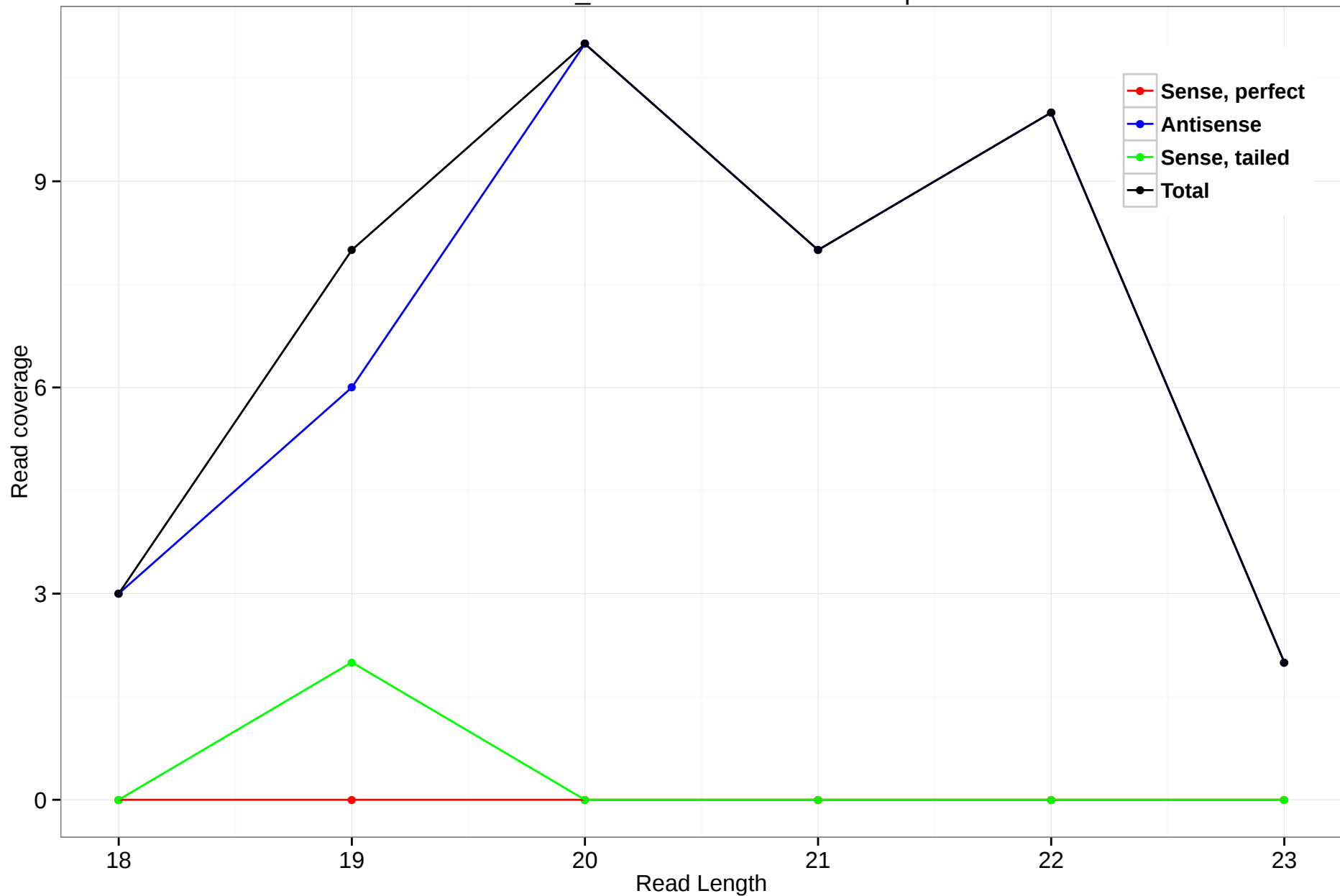
scaffold_4929:5729119-5730297.3p
