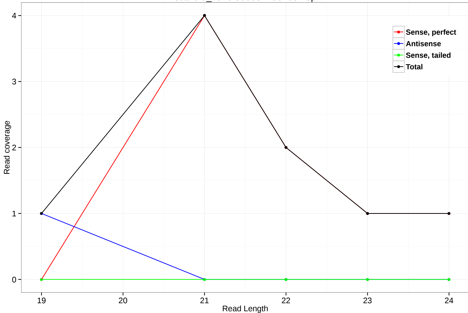
scaffold_4929:530331-531654.3p
