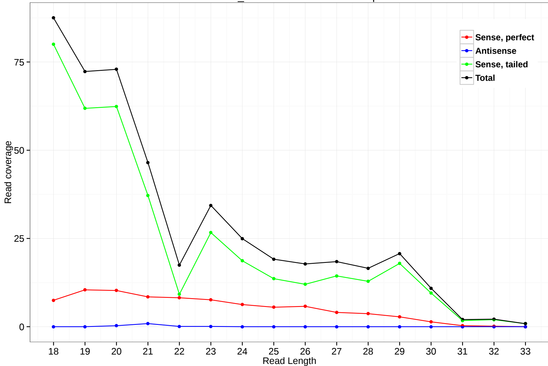
scaffold_4929:5300400-5320014.5p
