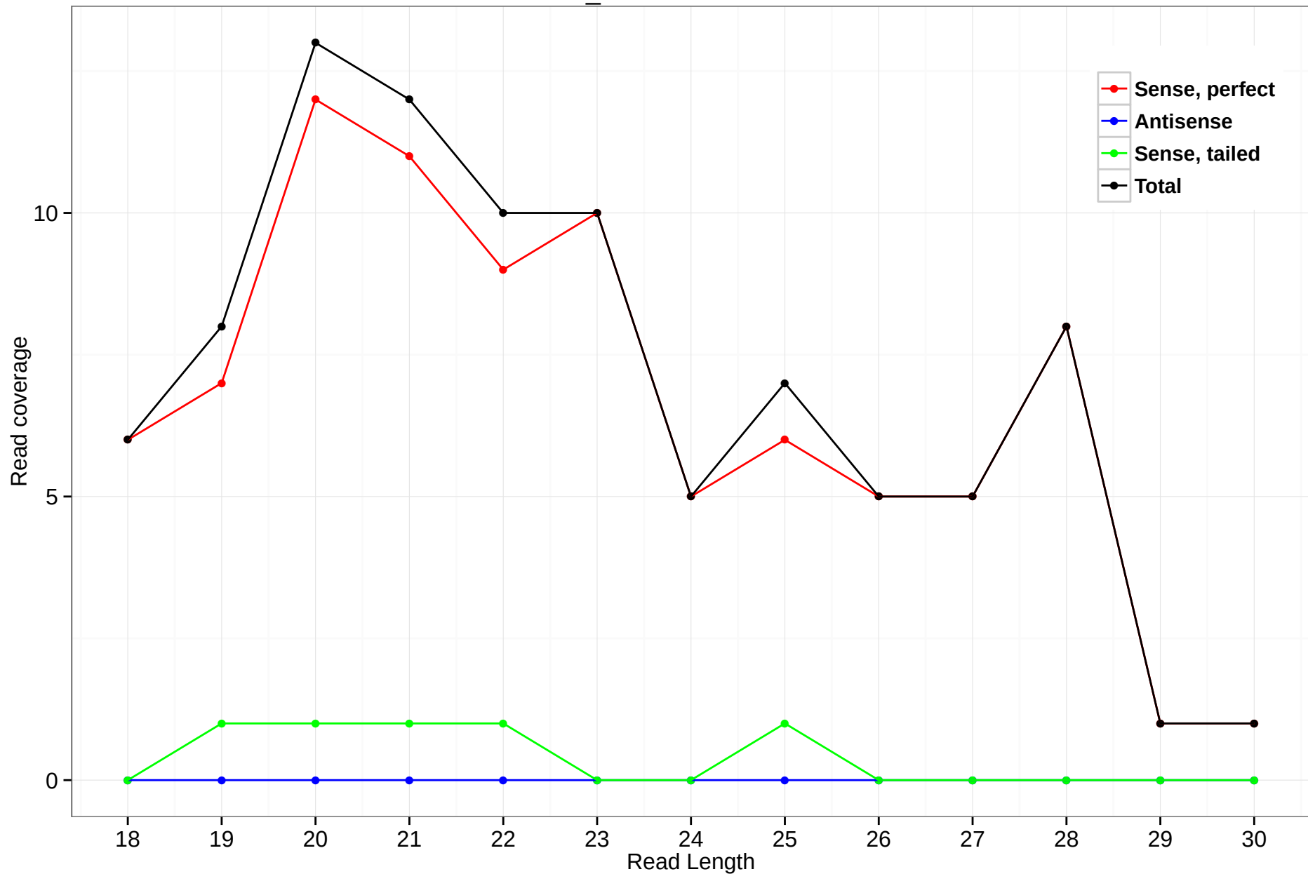
scaffold_4929:5283411-5283962
