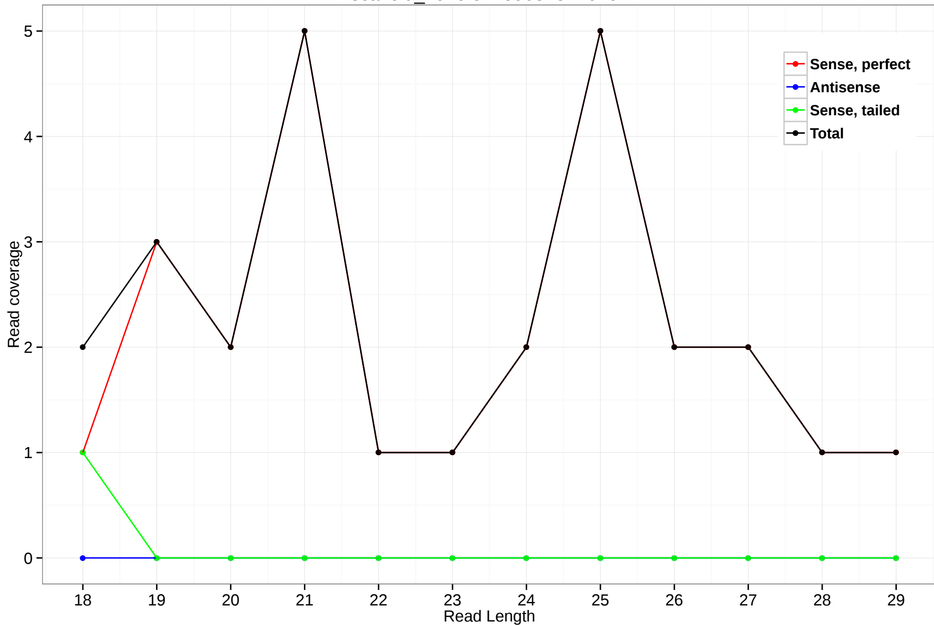
scaffold_4929:5125968-5126164
