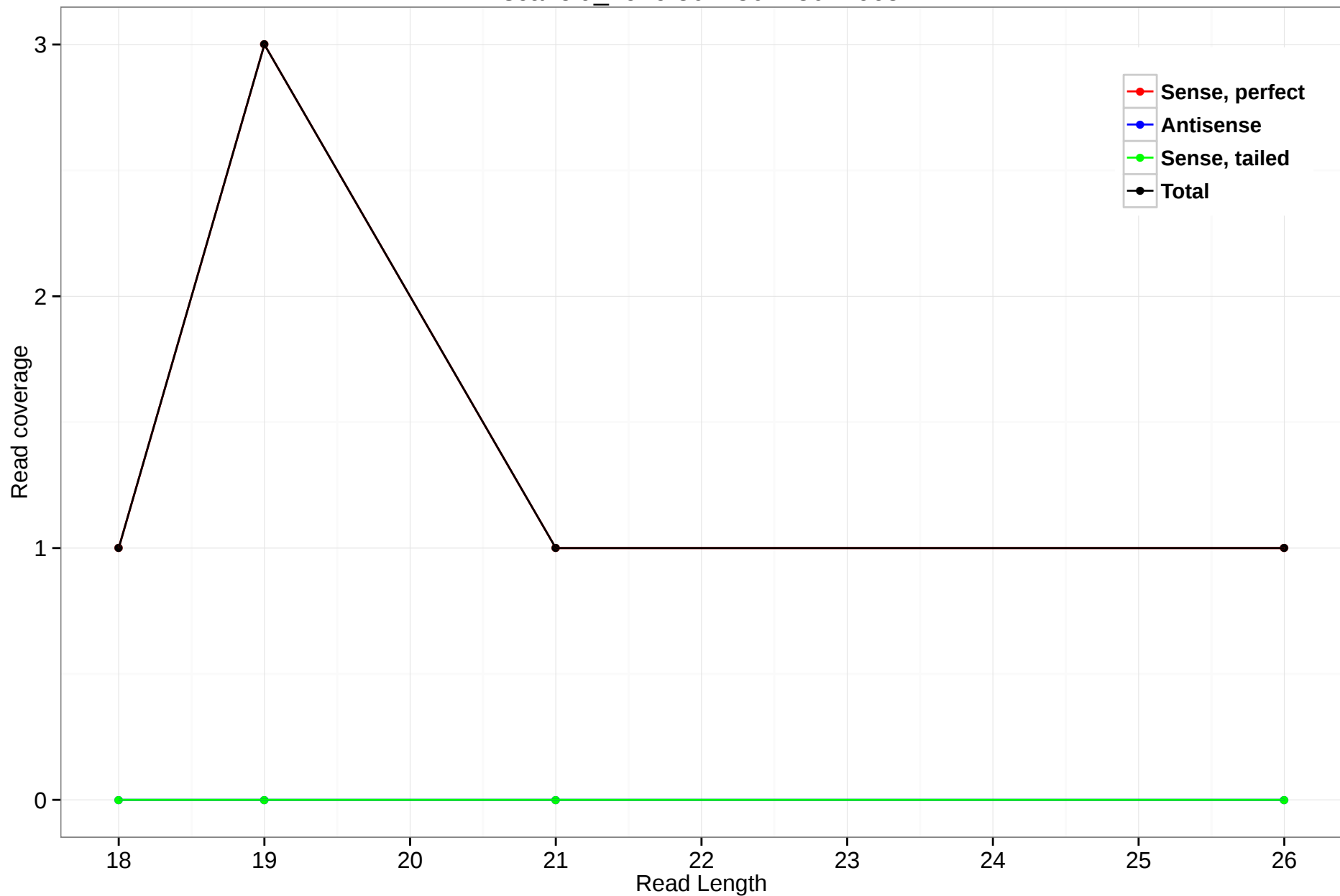
scaffold_4929:5072502-5072665
