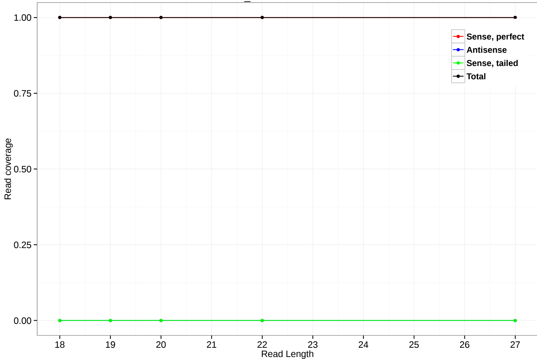
scaffold_4929:4910684-4910863
