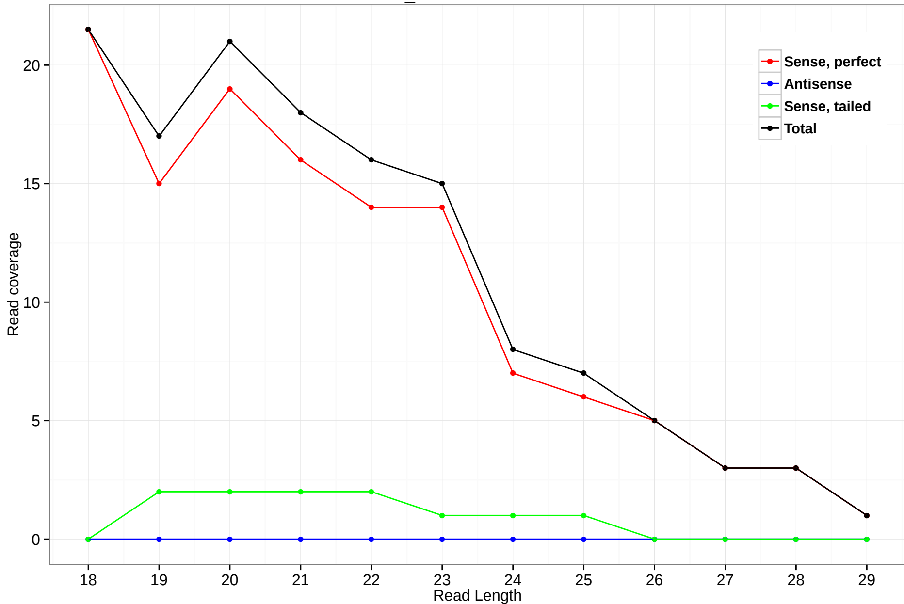
scaffold_4929:4545192-4545537
