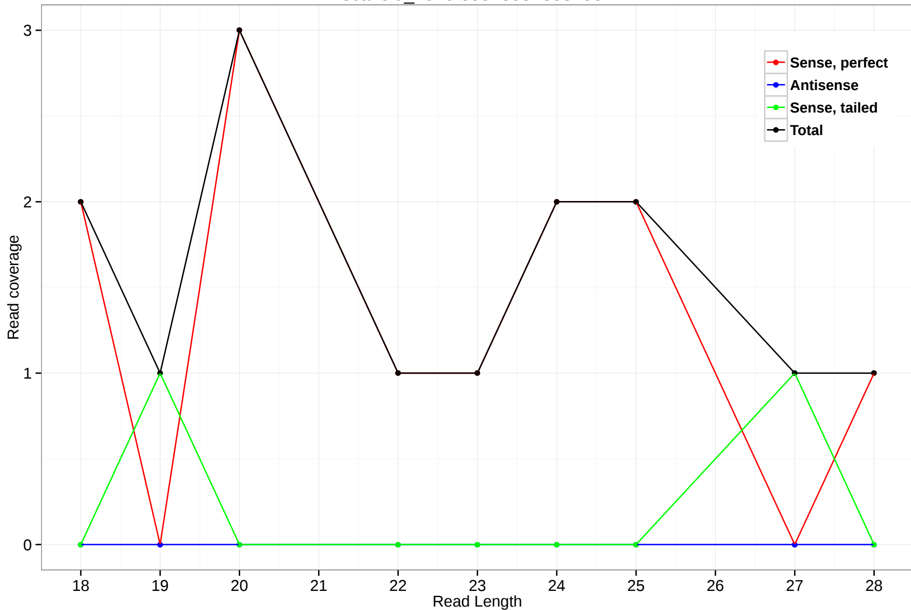
scaffold_4929:3534358-3534532
