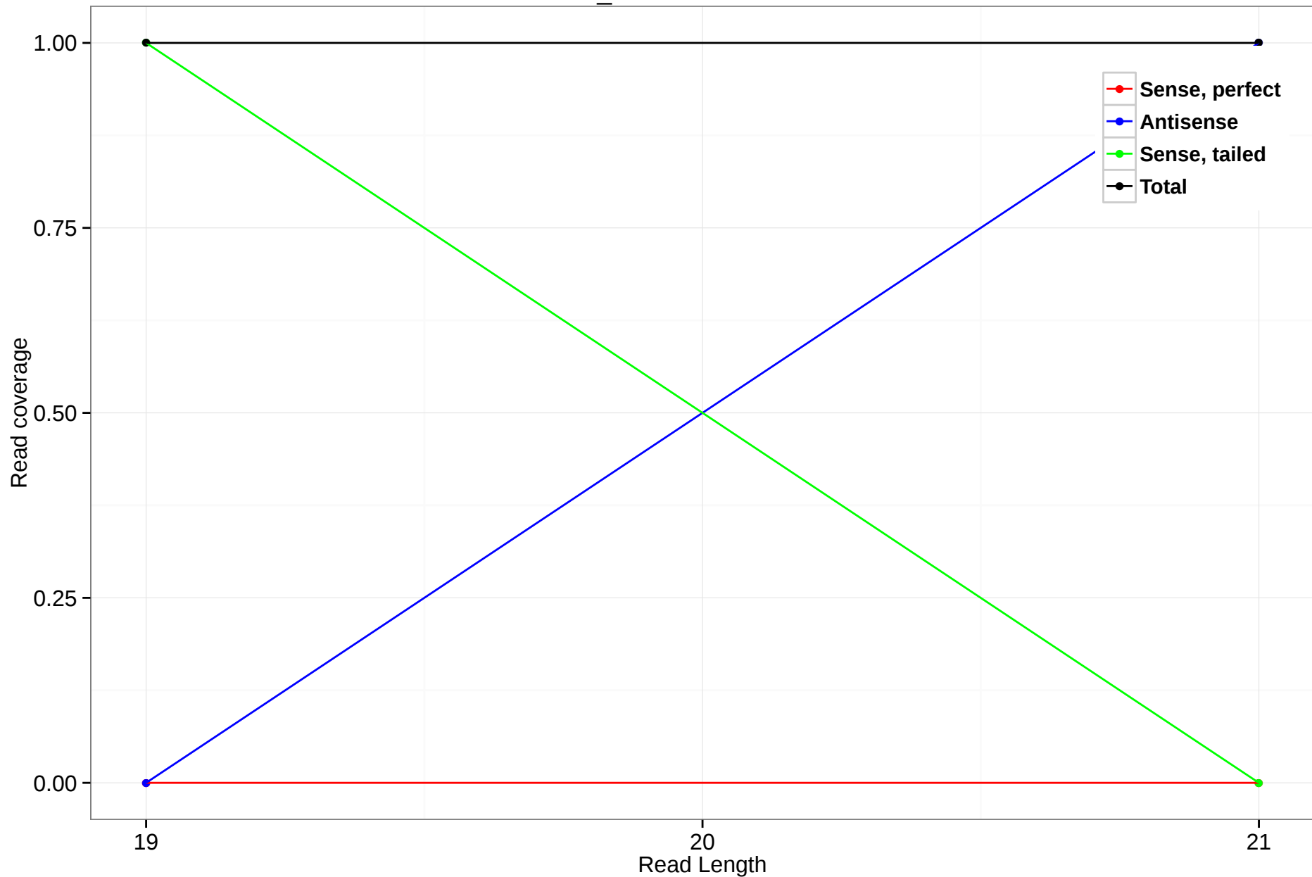
scaffold_4929:2817974-2818182
