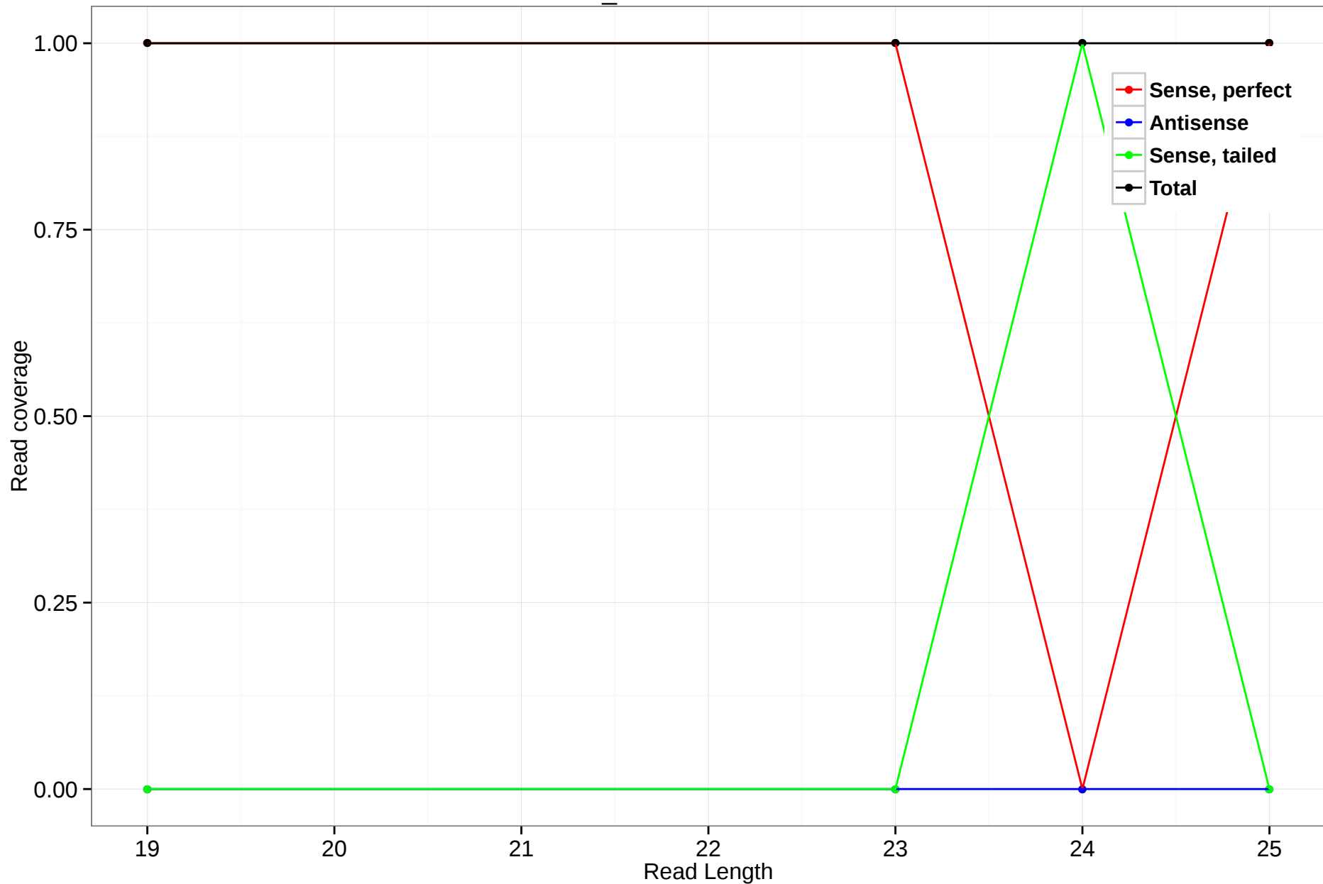
scaffold_4929:2790114-2790304
