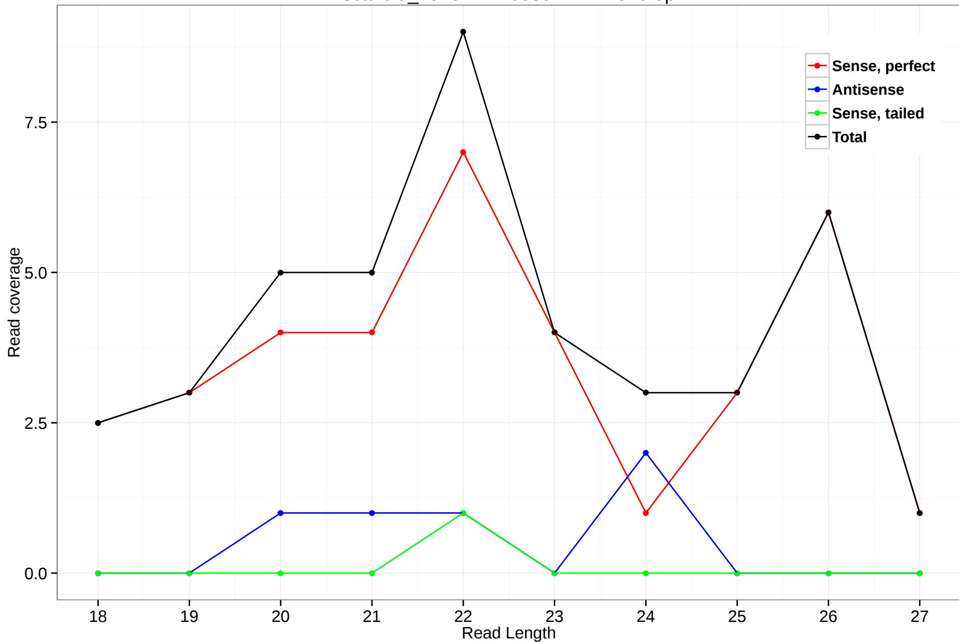
scaffold_4929:24716839-24717919.5p
