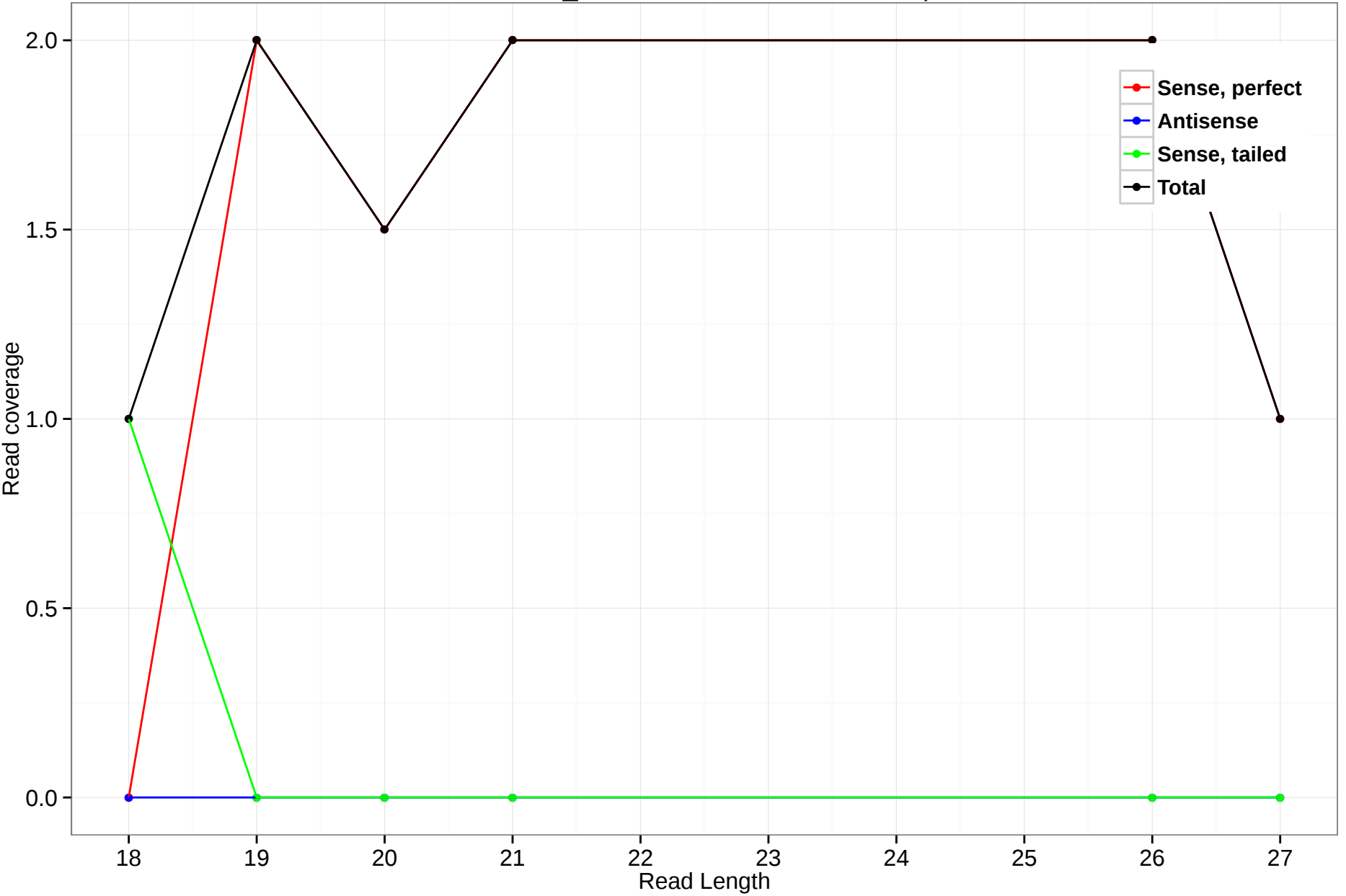
scaffold_4929:24646916-24681105.5p
