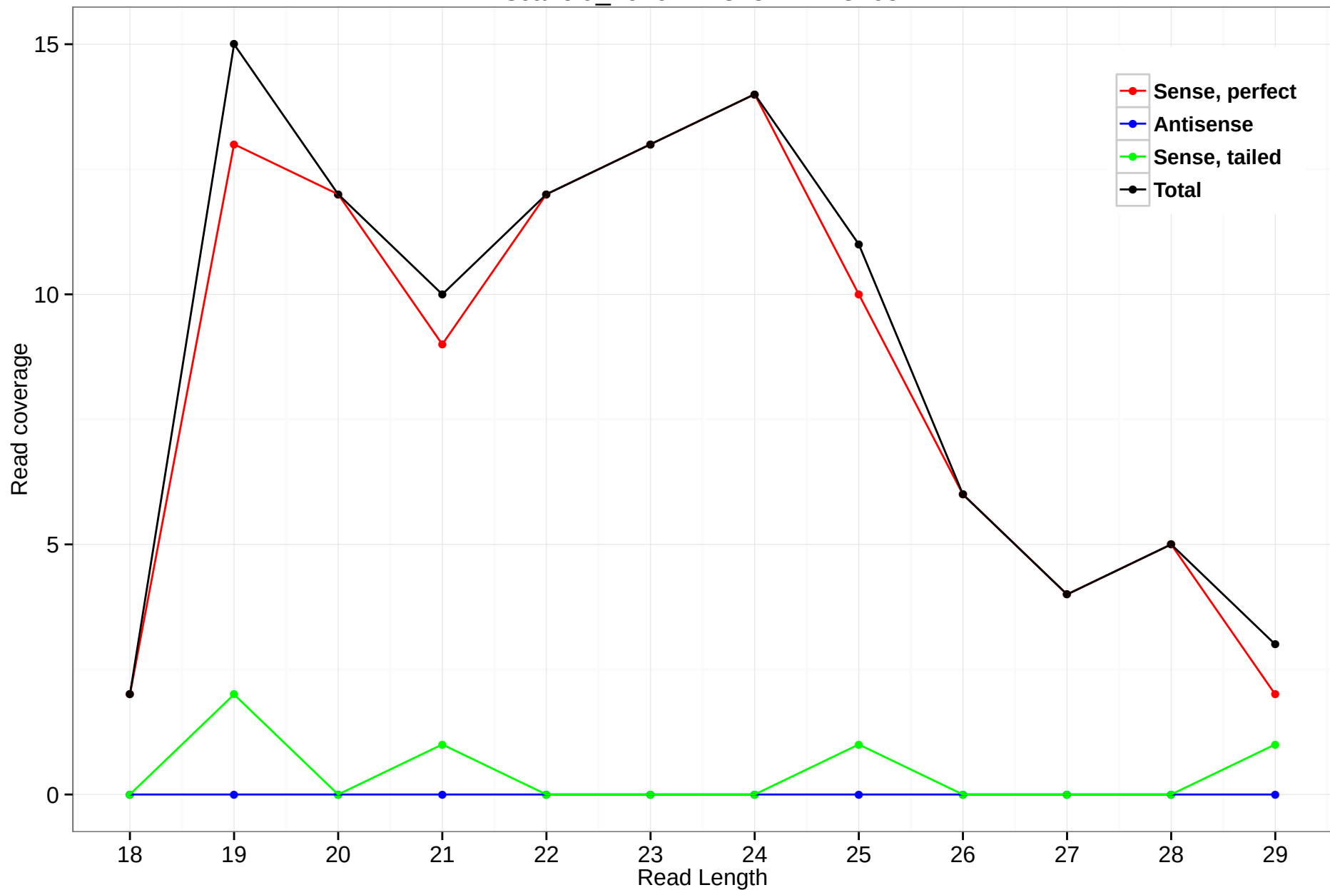
scaffold_4929:2413152-2413465
