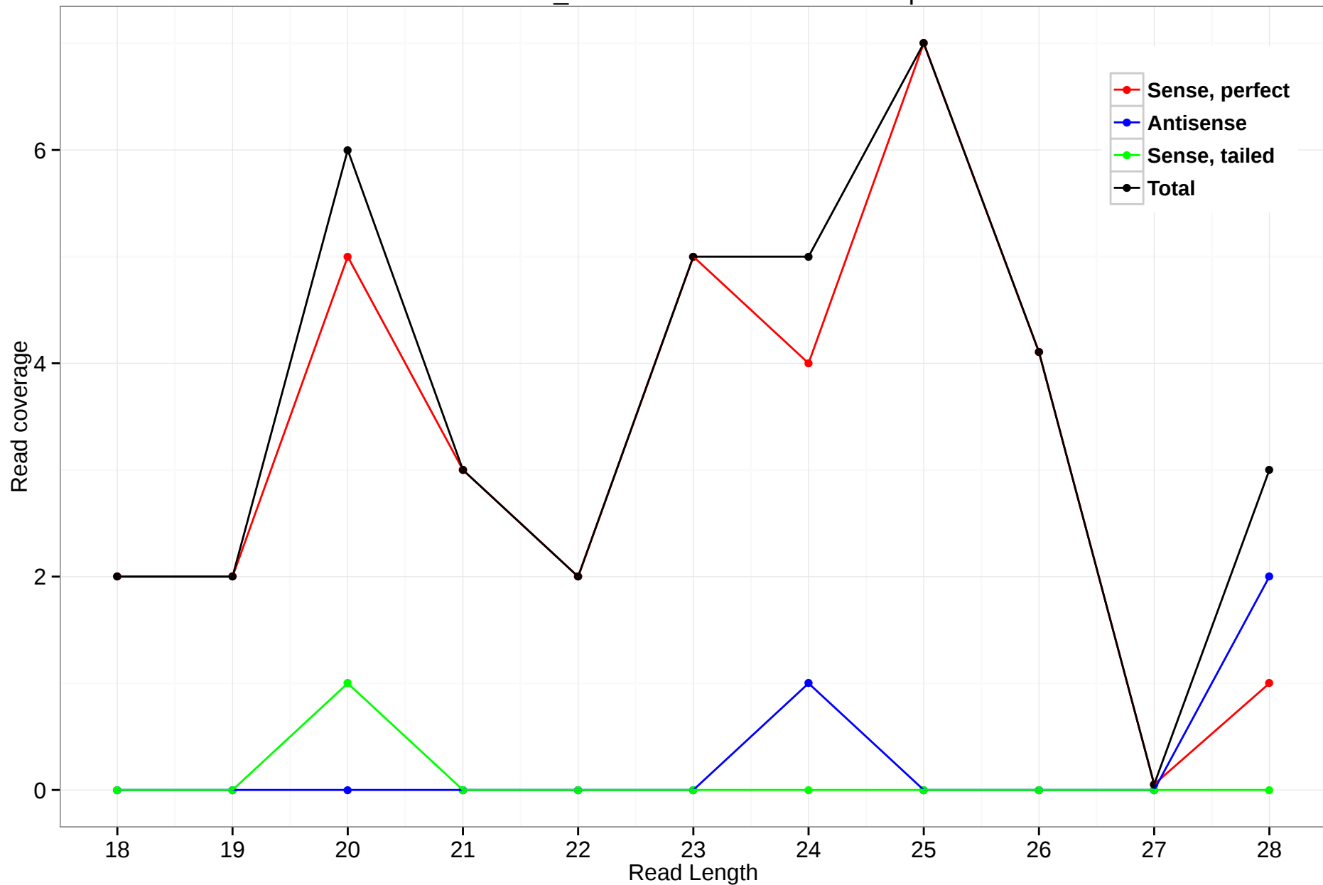
scaffold_4929:21790063-21796803.3p
