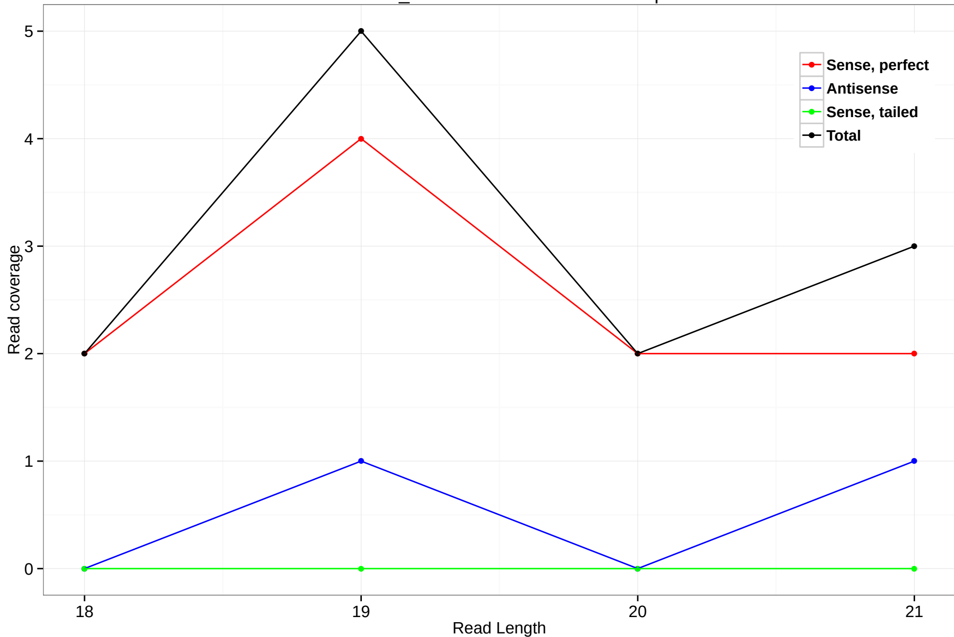
scaffold_4929:21532859-21536279.3p
