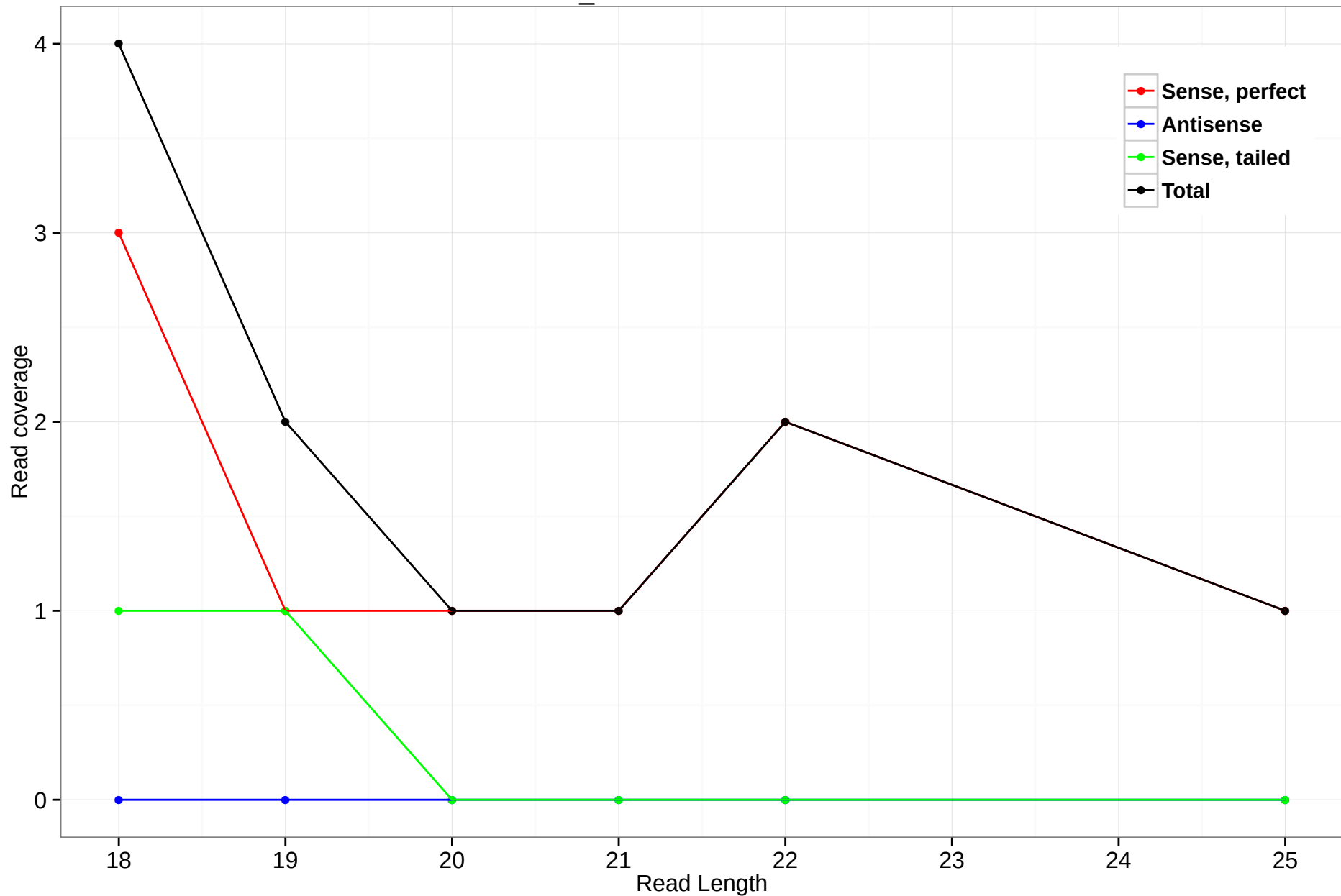
scaffold_4929:20816030-20816494
