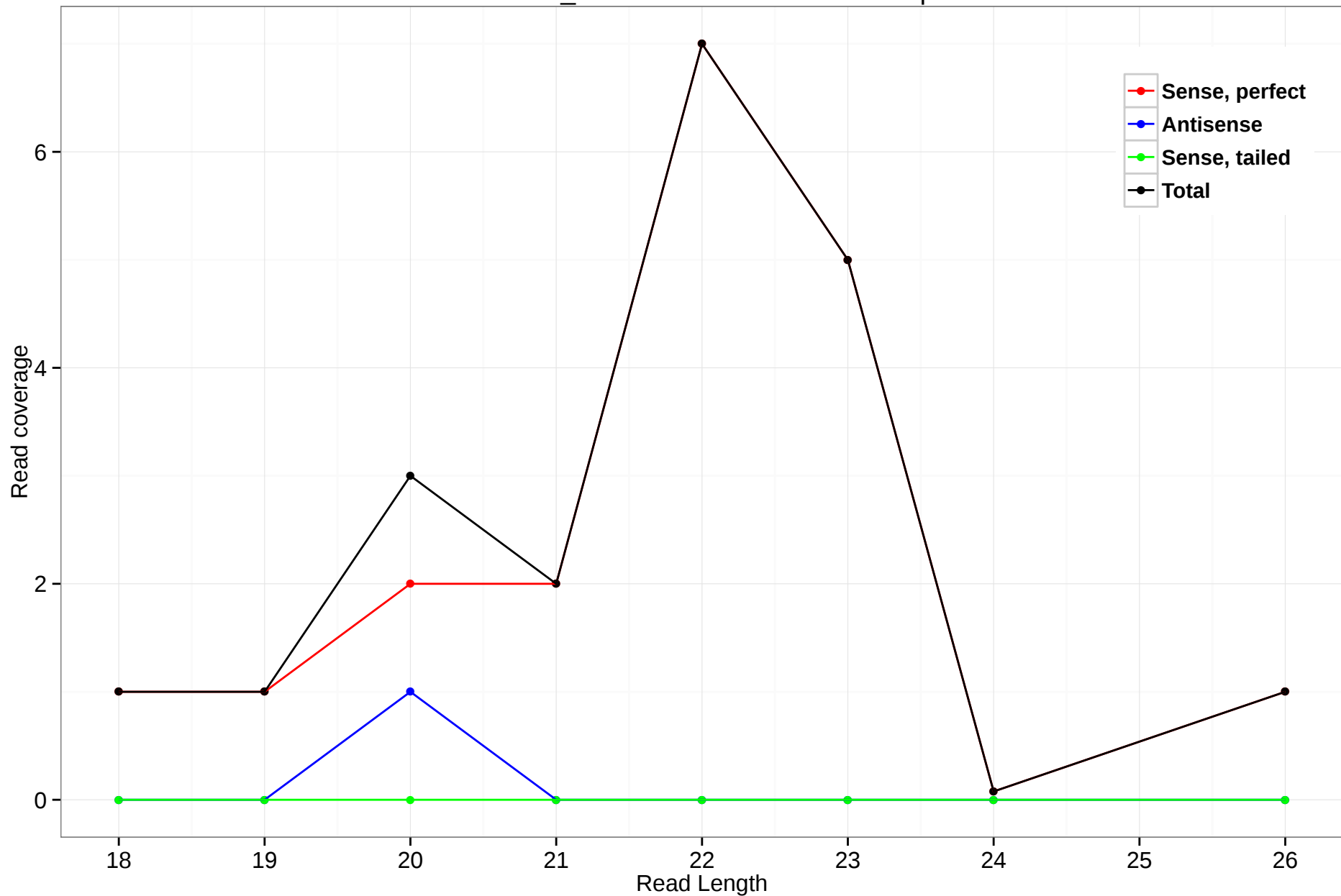
scaffold_4929:20182882-20183608.5p
