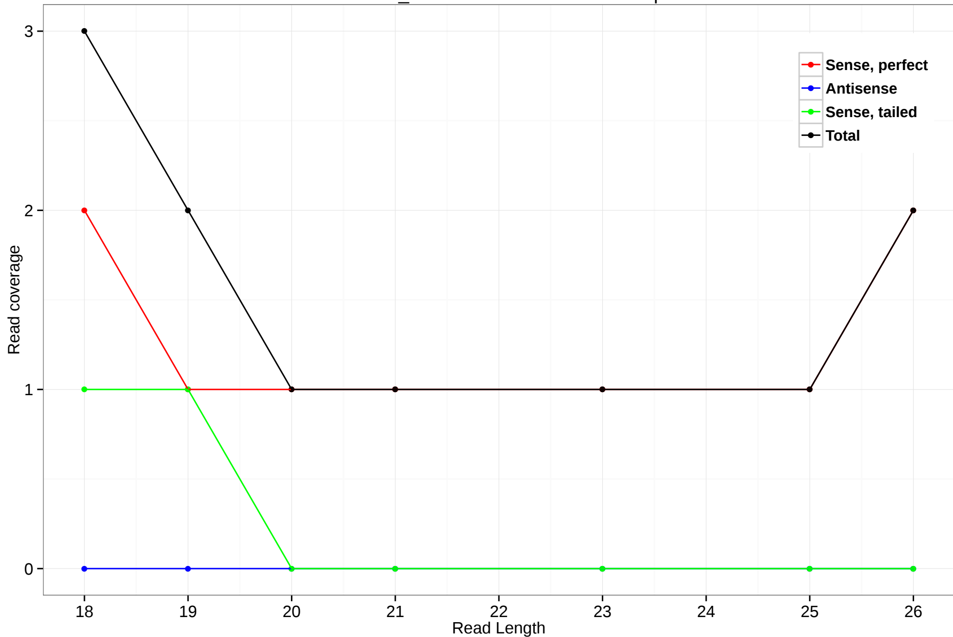
scaffold_4929:19988888-19989533.5p
