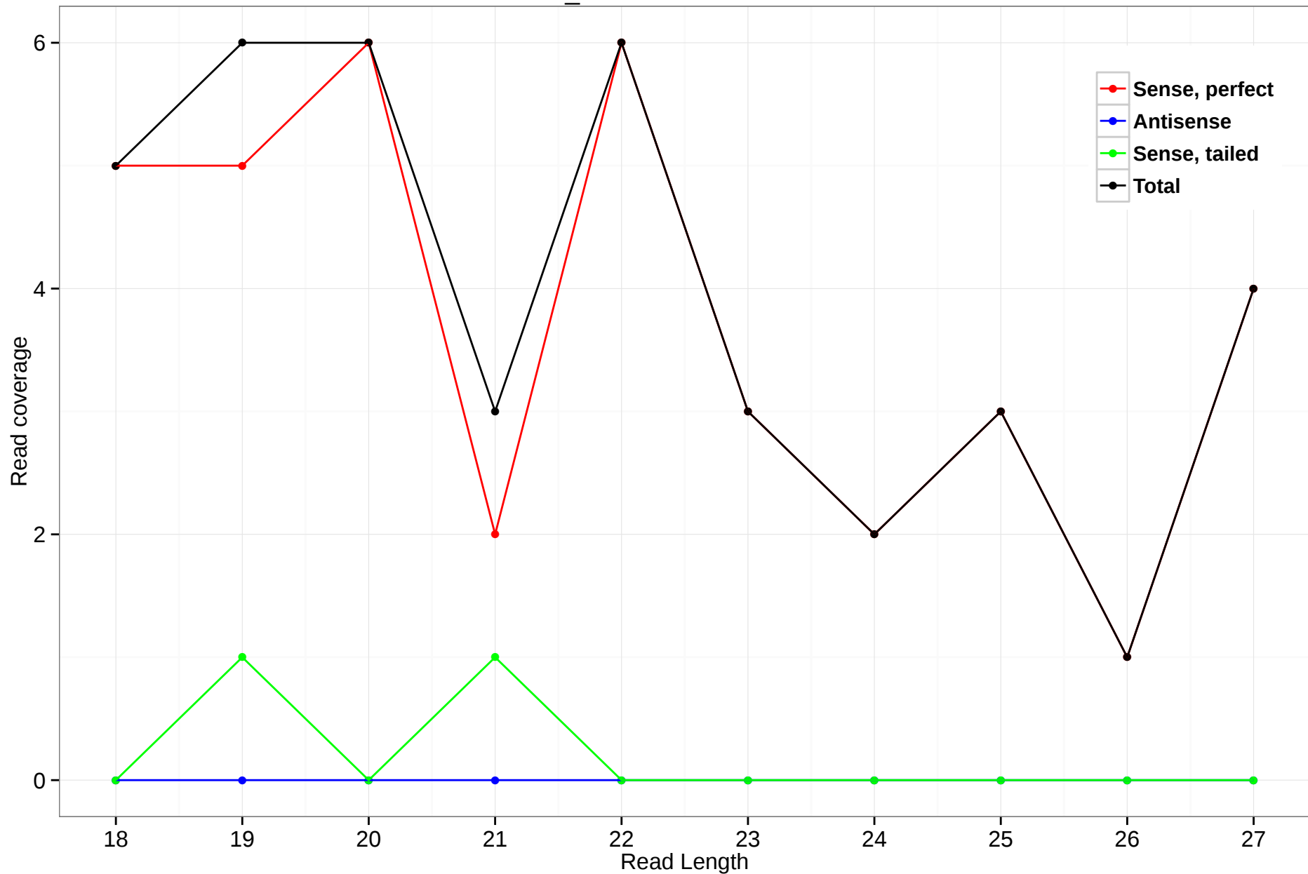
scaffold_4929:19660924-19661215
