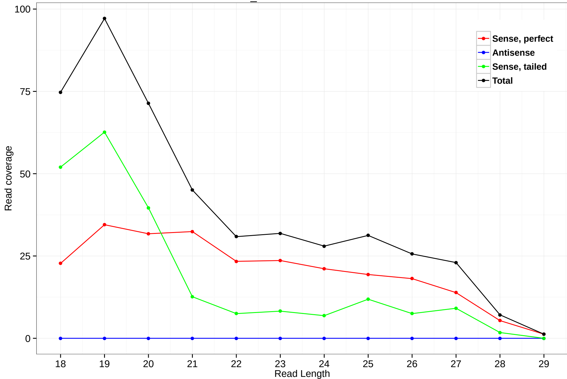
scaffold_4929:19609587-19609751
