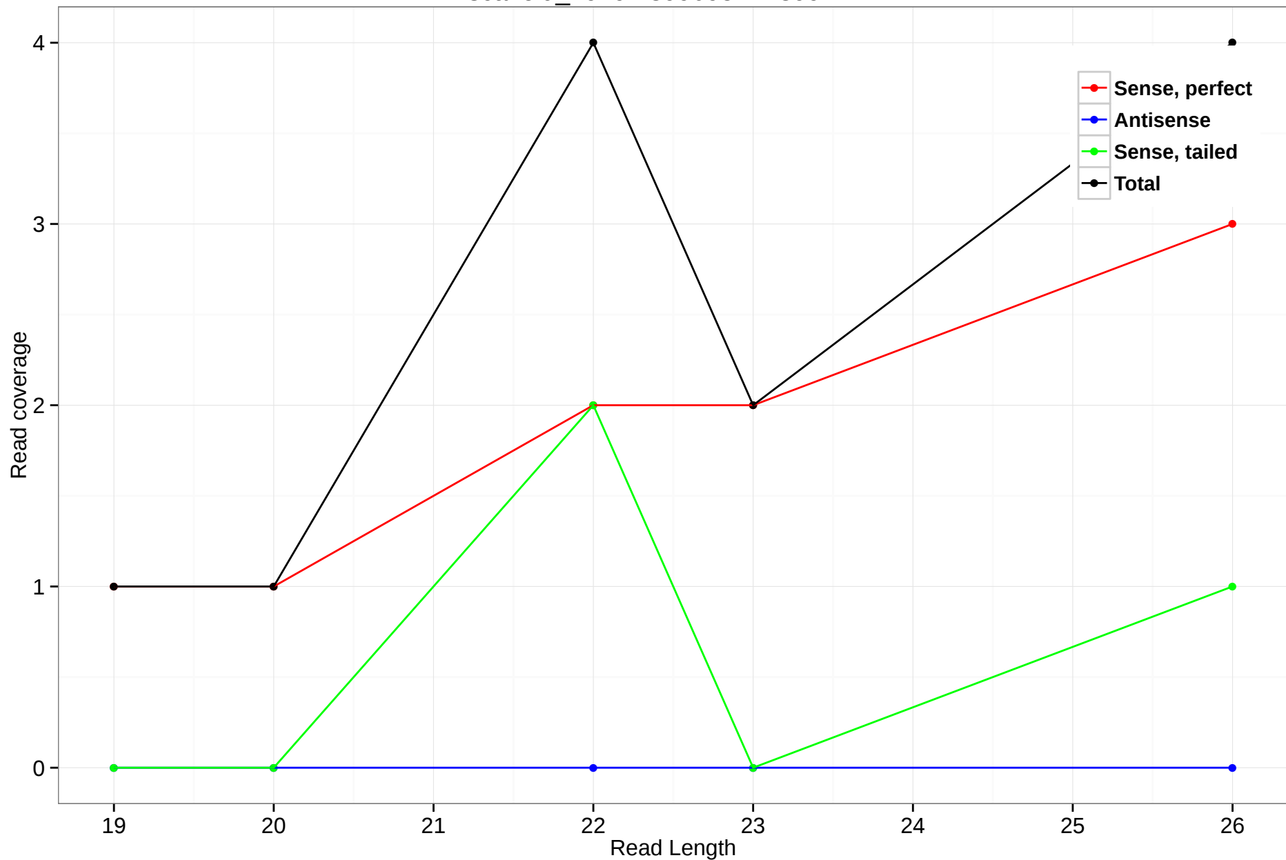
scaffold_4929:18990952-18991271
