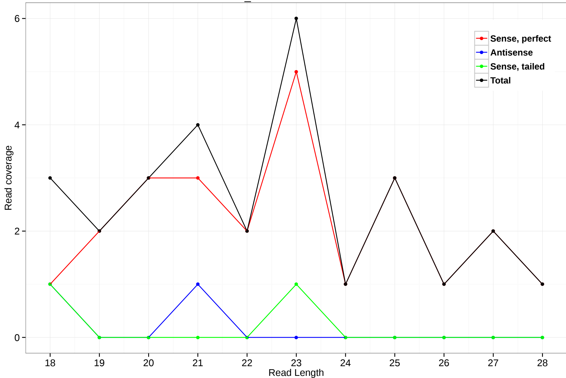
scaffold_4929:18906086-18906439
