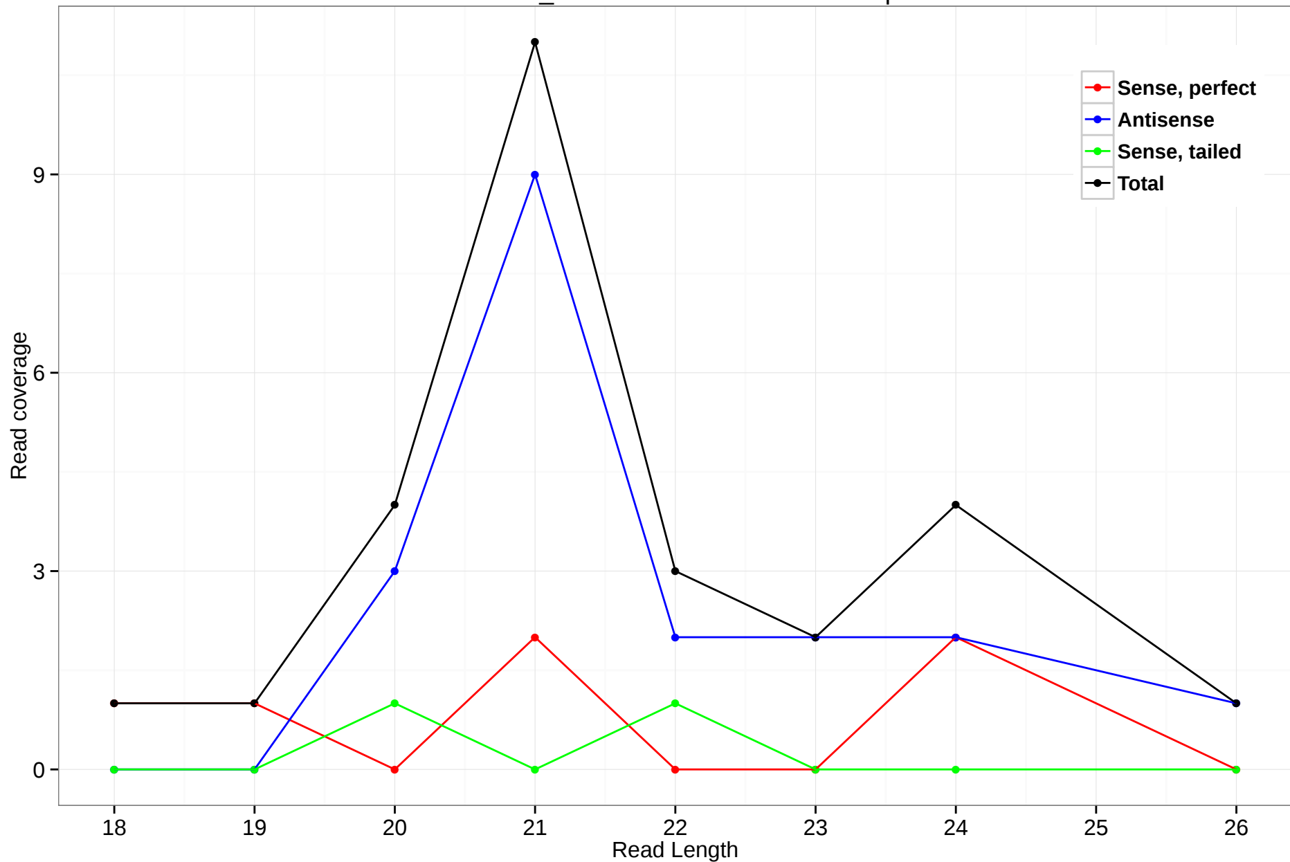
scaffold_4929:18733423-18735878.3p
