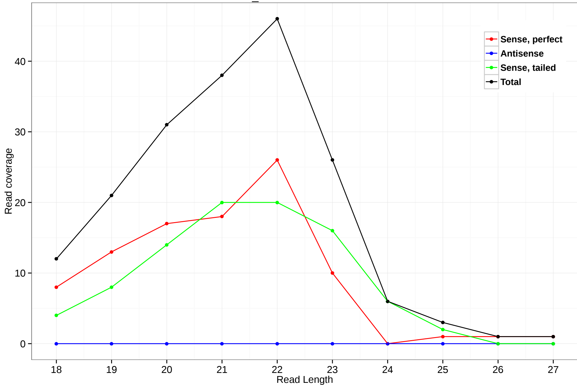
scaffold_4929:18305414-18305911
