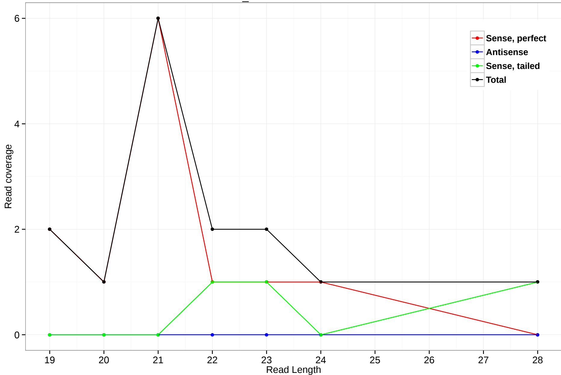
scaffold_4929:18301740-18301894
