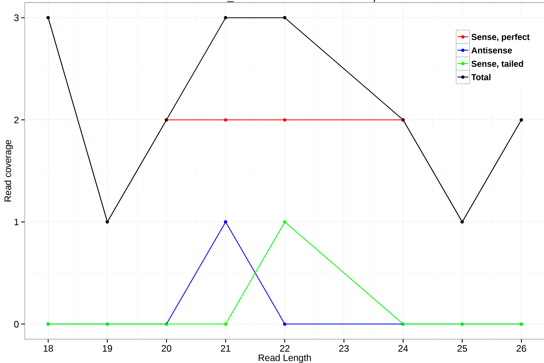
scaffold_4929:17860004-17860962.5p
