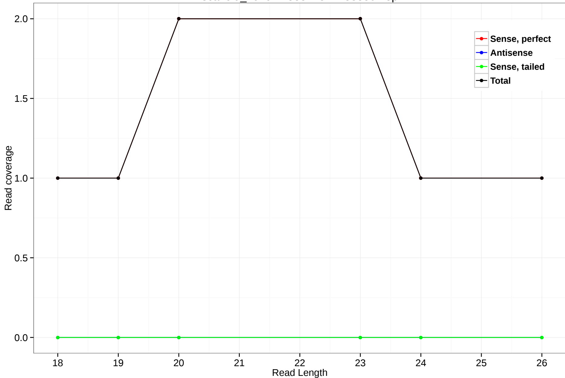
scaffold_4929:17583275-17588501.3p
