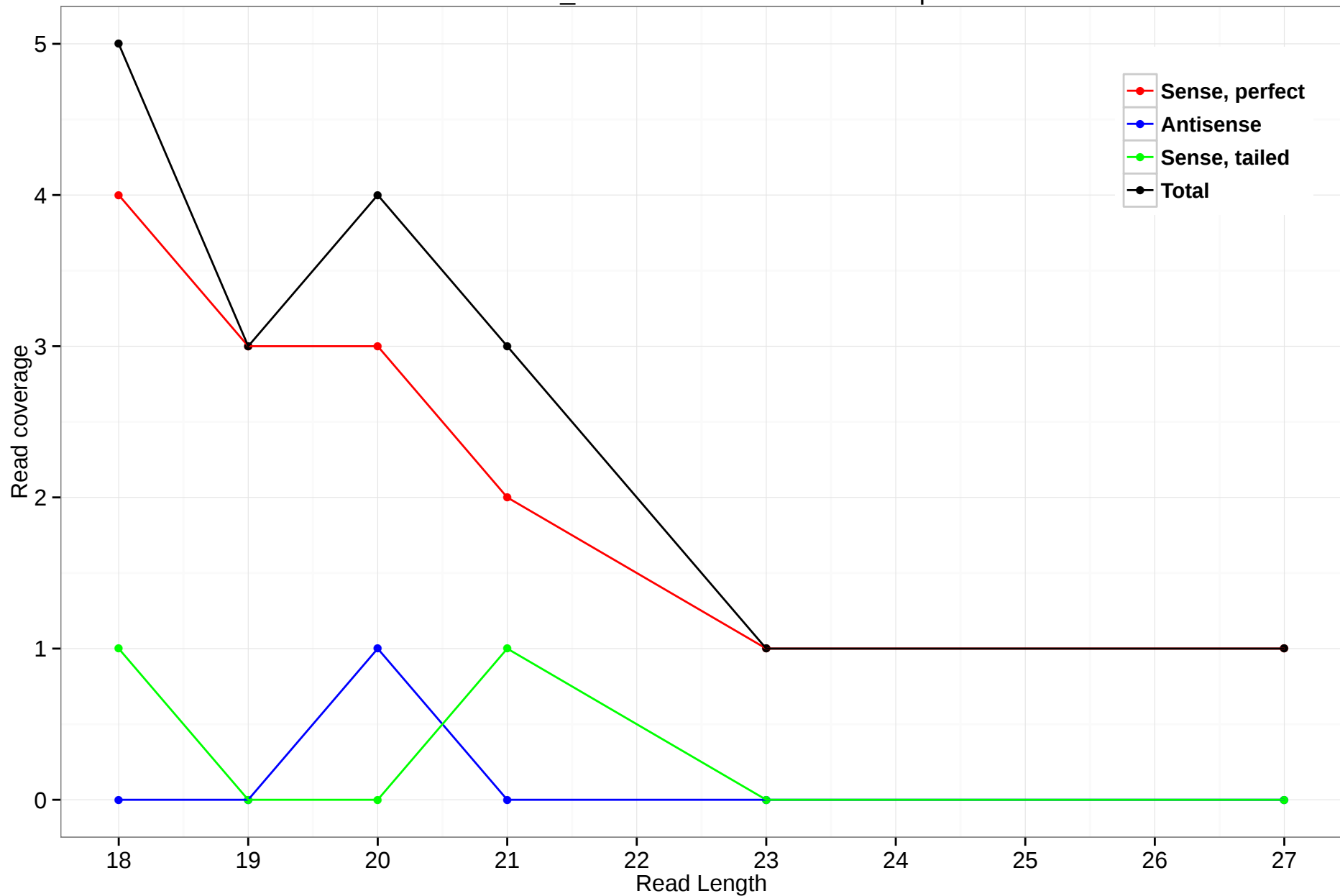
scaffold_4929:17580385-17581195.3p
