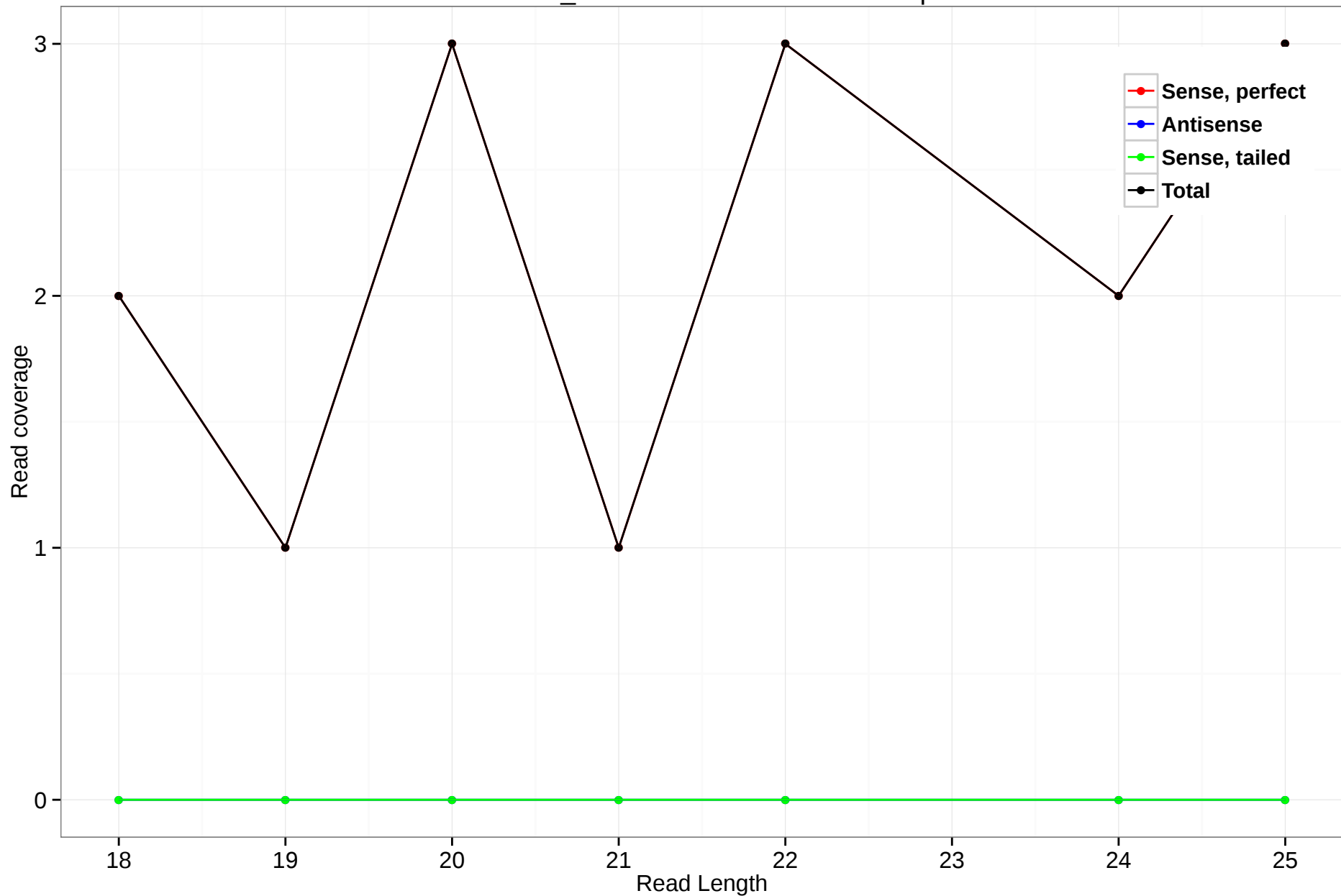
scaffold_4929:17267501-17268663.3p
