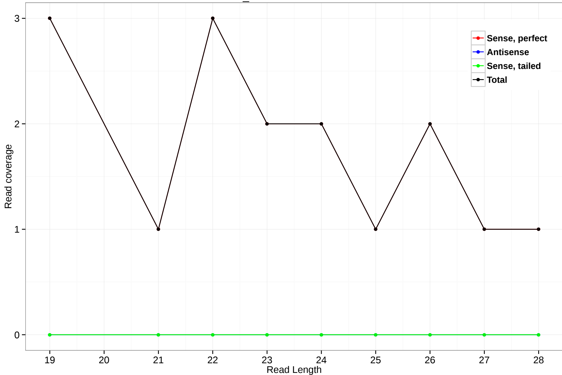
scaffold_4929:16656225-16656503
