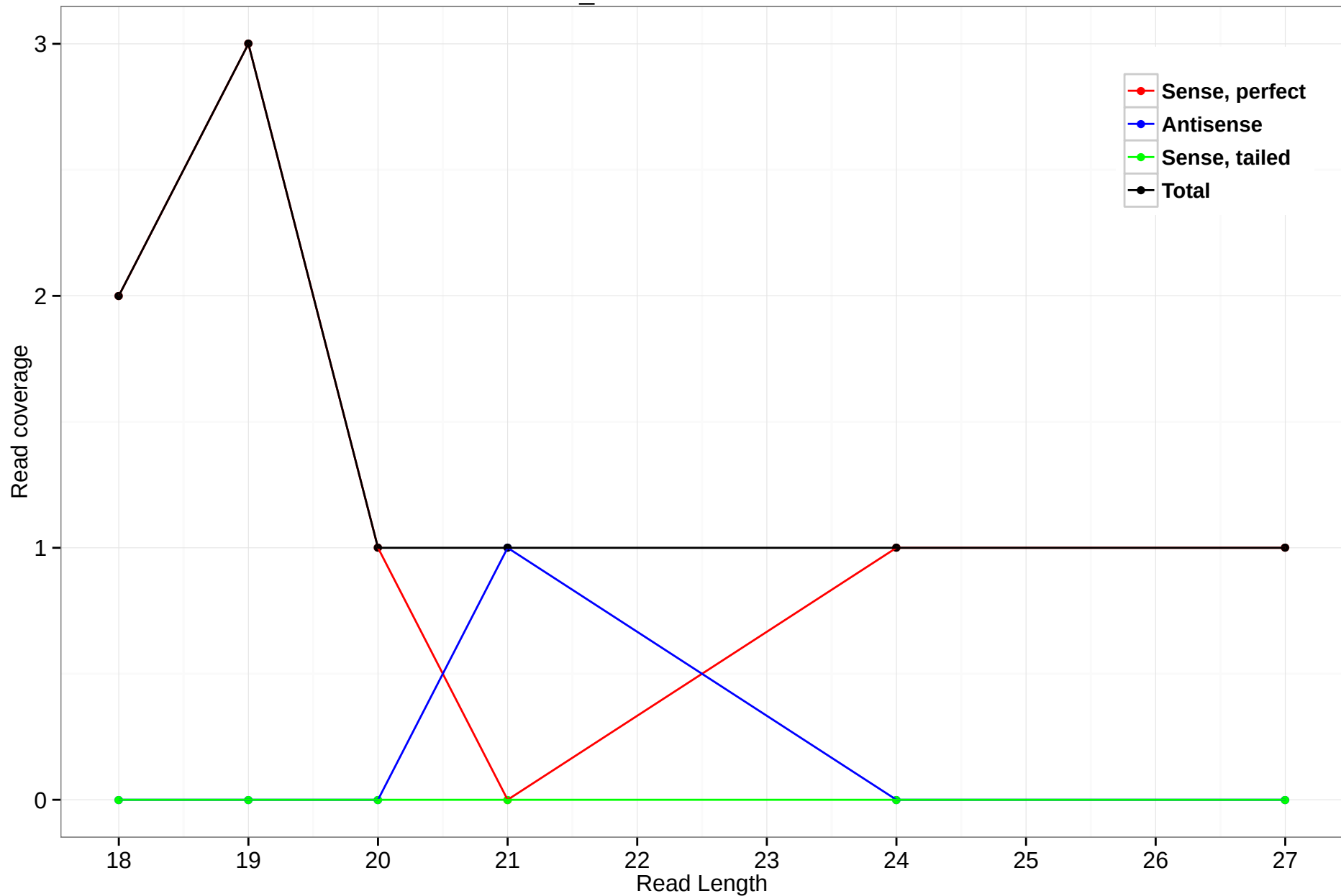
scaffold_4929:15935796-15936069
