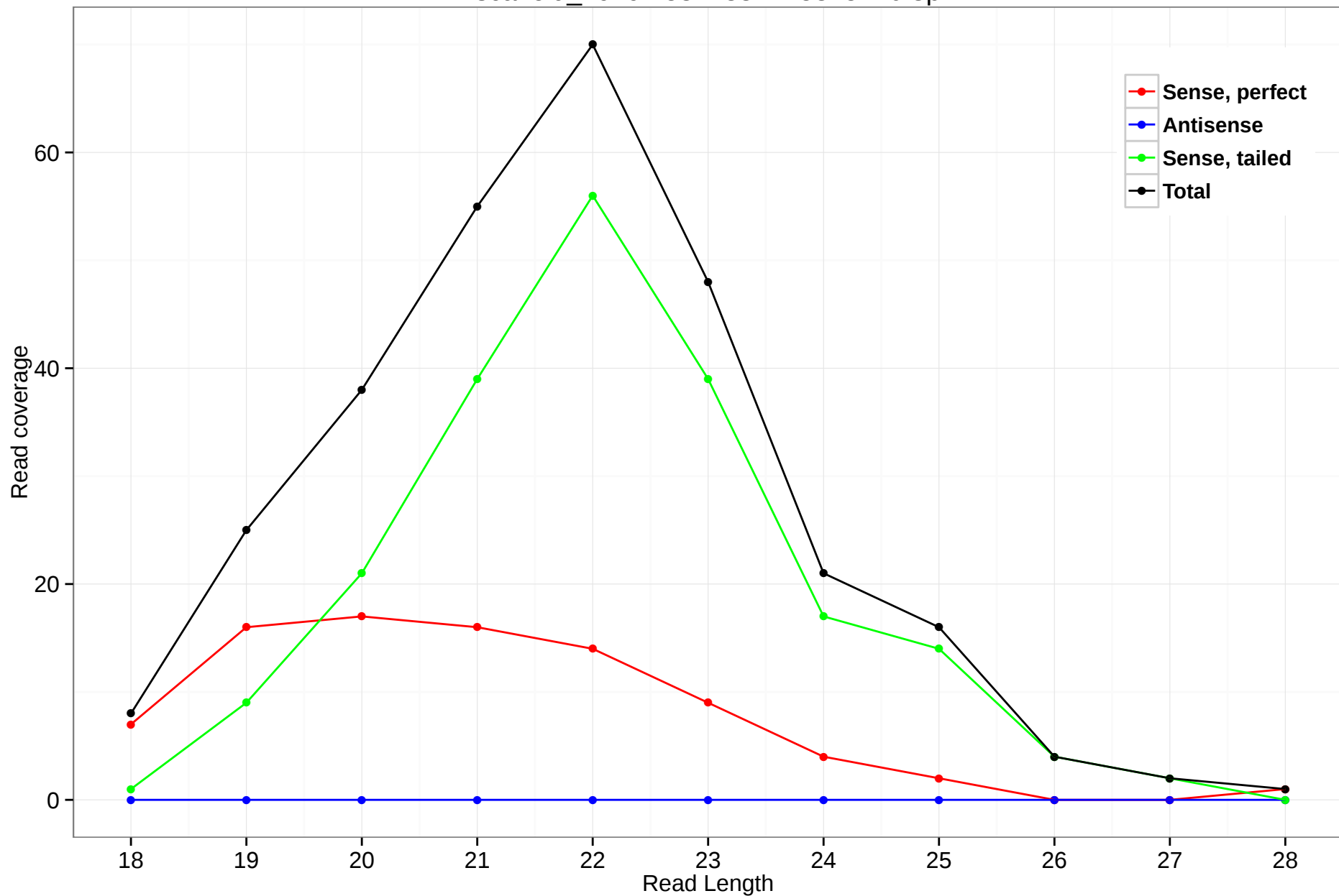
scaffold_4929:15814881-15815770.3p
