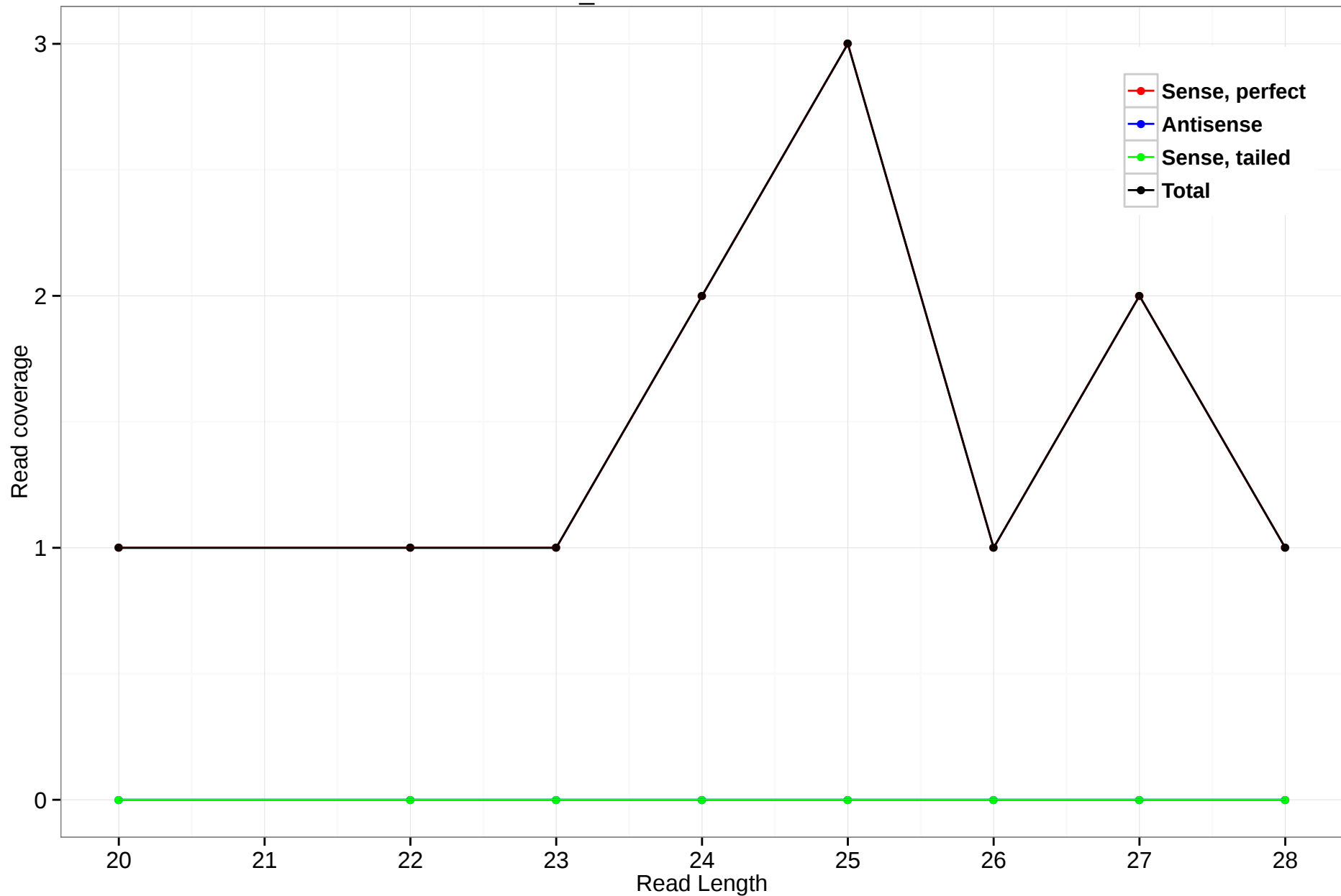
scaffold_4929:15543831-15544036
